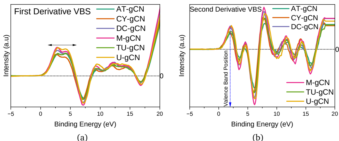
Figure 4.21: Derivative valence band XPS plots and valence band position estimation through the second derivative method for carbon nitrides.
