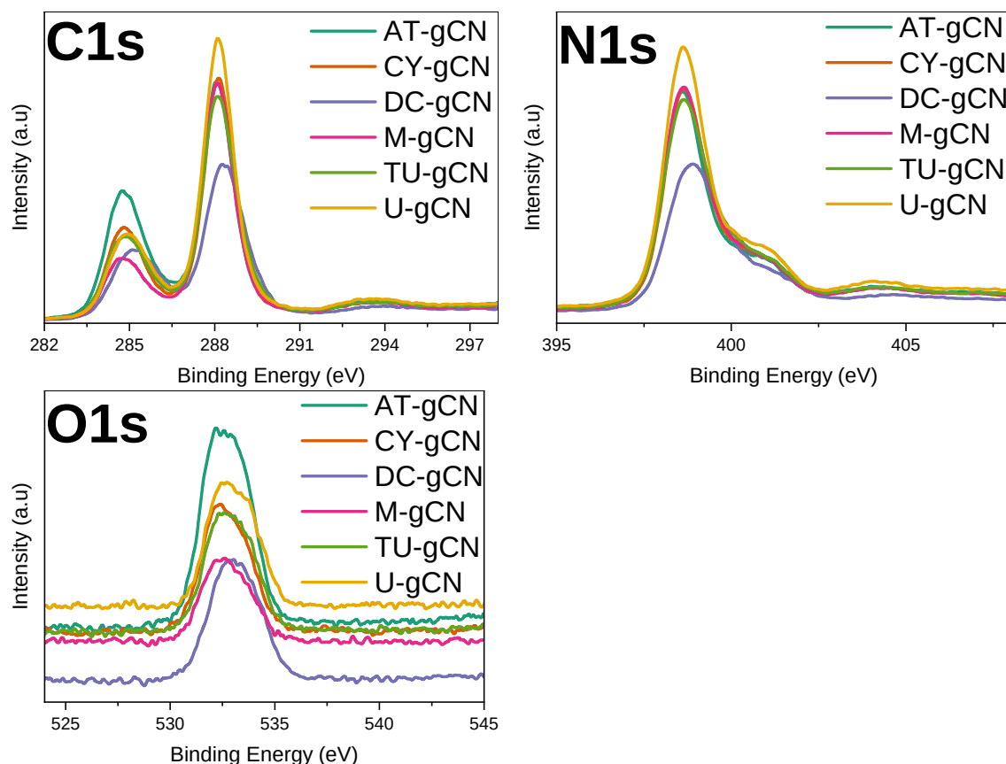
Figure 4.18: C1s , N1s , and O1s photoelectron spectra of graphitic carbon nitriles
