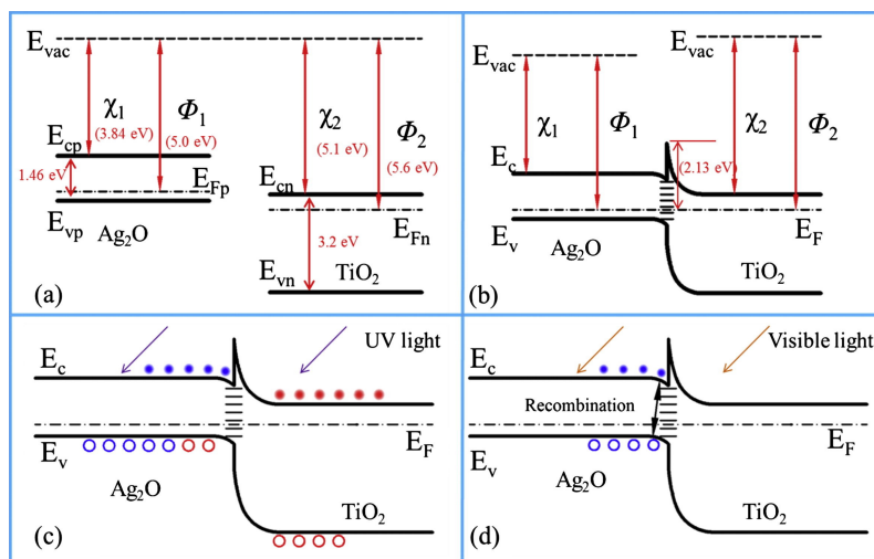
Figure 2.29: (a) Energy band structures of \text{Ag}_2\text{O} and \text{TiO}_2 before the formation of the nanoheterojunction. (b) Energy band structures of the p- \text{Ag}_2\text{O} /n- \text{TiO}_2 nano-heterojunction at the equilibrium state. (c) Energy band structures of the p- \text{Ag}_2\text{O} /n- \text{TiO}_2 nano-heterojunction upon UV irradiation. (d) Energy band structures of the p- \text{Ag}_2\text{O} /n- \text{TiO}_2 nano-heterojunction upon visible light irradiation [178]. Reproduced from J. Colloid Interface Sci. 492 (2017) 167–175. ©2017 Elsevier B.V.
