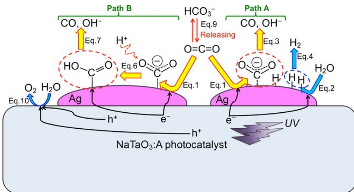
Figure 2.40: The proposed mechanism for CO 2 reduction to form CO over Ag/NaTaO 3 photocatalysts involving Path A [hydrogenation of \bullet\text{CO}_2^- ] and Path B [reduction of \text{COOH}_{(ad)} ] is discussed. The photocatalysts used were A=Mg, Ca, Sr, Ba, and La [255]. Reproduced from ChemSusChem . 10 (2017) 112–118. ©2017 Wiley-VCH Verlag GmbH & Co. KGaA, Weinheim.
