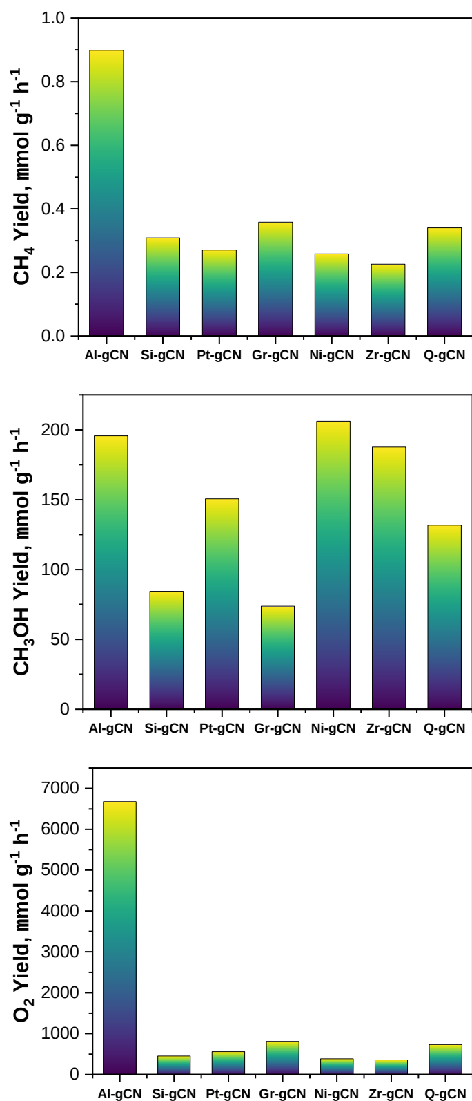
Figure 5.1: Product yields from the reduction of CO 2 over graphitic carbon nitriles, synthesized using various crucibles, activity reported with respect to total surface area.
