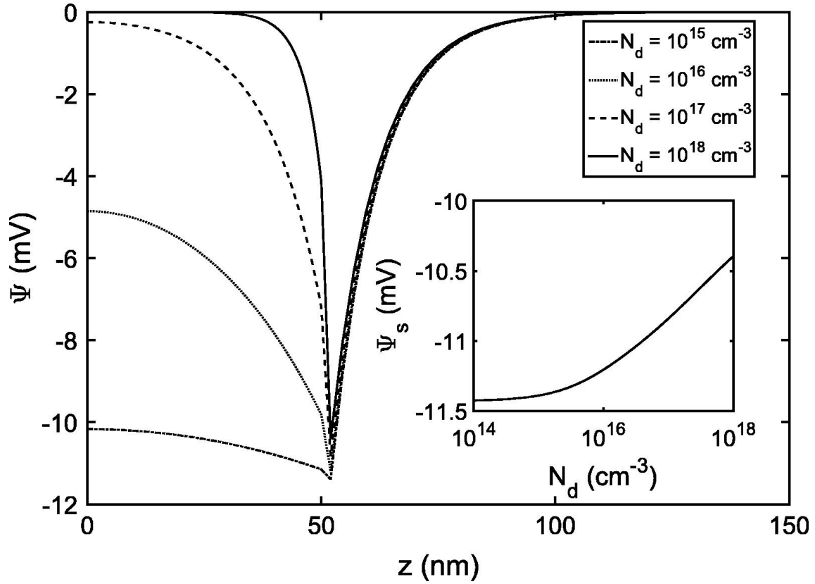
Figure 2.28: The potential distributions were graphed in relation to the distance z . The semiconductor/oxide interface was located at z = 50 \text{ nm} , whereas the oxide/electrolyte interface was located at z = 52 \text{ nm} . The pH of the electrolyte solution was adjusted to 3. The different lines indicate the varying doping concentrations. The inset shows a plot of the surface potential \Psi_s versus N_d doping. The potential distributions are plotted for a constant N_d doping level of 10^{18} \text{ cm}^{-3} . Additionally, the inset shows a plot of the surface potential \Psi_s in relation to the Debye length \kappa^{-1} [167]. Reproduced from J. Colloid Interface Sci. 449 (2015) 409–415. ©2015 Elsevier B.V.
