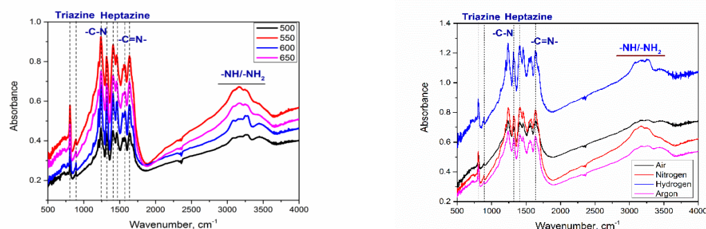
Fig.1. FTIR spectra of prepared graphitic carbon nitride at various temperatures and atmospheric conditions.
