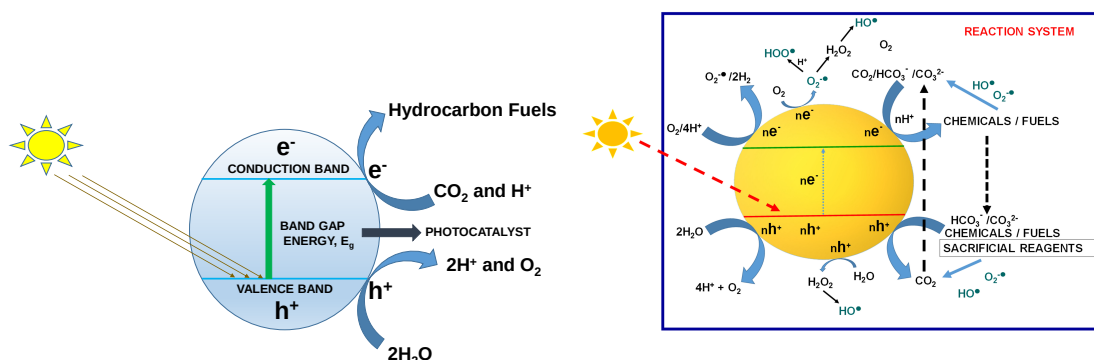
Figure 2.3: Illustrate the mechanisms of gaseous phase CO 2 reduction and the possible reactions involved in the CO 2 reduction process, respectively [11]. Reproduced from Indian J. Chem. Sec. A 56 (2017) 251–269. ©2017 Council of Scientific and Industrial Research–National Institute of Science Communication and Policy Research, India.
