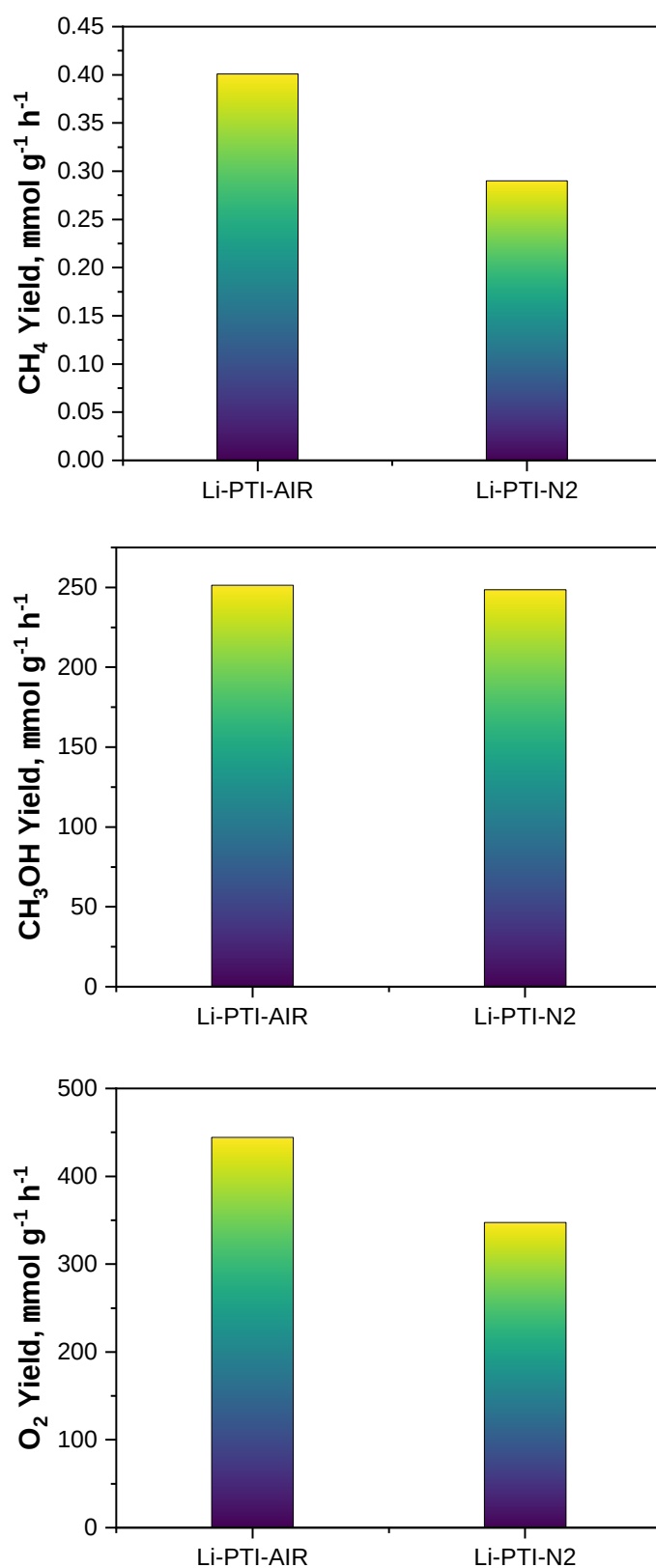
Figure 6.1: Product yields from the reduction of \text{CO}_2 over Li-PTI samples, activity reported with respect to total surface area.
