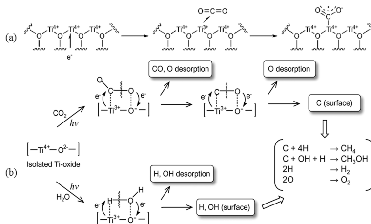
Figure 2.24: (a) The process by which CO 2 molecules are adsorbed and subsequently converted into \text{•CO}_2^- species on TiO 2 surfaces, as well as the concurrent formation of these species [110]. Reproduced from Chem. Rev. 115 (2015) 12888–12935. ©2015 American Chemical Society (b) Photoreduction of CO 2 to the reduced forms of anchored TiO 2 species [111]. Reproduced from RSC Adv. 2 (2012) 3165. ©2012 Royal Society of Chemistry.
