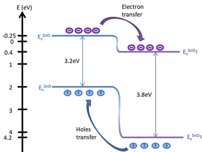
Figure 1.8 Schematic representation of charge carrier behavior in type II heterostructure ZnO/ \text{SnO}_2 . Reproduced from [20].
