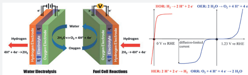
FIGURE 6 —Scheme of PEMFC and PEMEC, and polarization curves of the main electrode reactions. Sources: S. Park, Y. Shao, J. Liu, Y. Wang, Energy Environ. Sci. (2012) 5, 9331; Y. Jiao, Y. Zheng, M. Jaroniec, S.Z. Qiao, Chem. Soc. Rev. (2015) 44, 2060. With due permissions.
