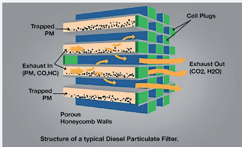
FIGURE 3 –Honeycomb system treating gases and soot from industrial Diesel motors. Source: http://urbanemissions.blogspot.com/2015/12/what-is-diesel-particle-filter-dpf.html .
