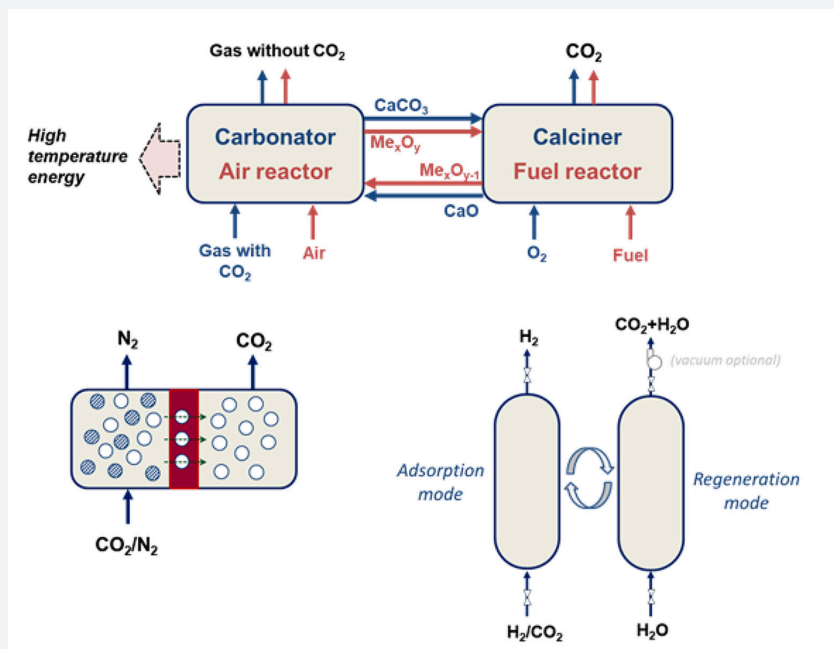
FIGURE 1 —Emerging CO 2 capture technologies (upper figure: high temperature looping solid technologies (red lines: CLC and blue lines: Ca-Looping). Bottom figures: membranes and adsorption technologies; gas mixtures chosen for comparison purposes, other mixtures could be possible).
