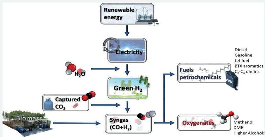
FIGURE 5 —Possible routes for renewables-to-SG-to-products processes. Source: freely elaborated and adapted by M.A. Centeno with a student of his, starting from Z. Jiang, T. Xiao, V. L. Kuznetsov, P. P. Edwards: Phil. Trans. R. Soc. A (2010) 368, 3343; and G. Leonzio: Waste and Biomass Valorization , doi: 10.1007/s12649-019-00914-4. With due permissions.
