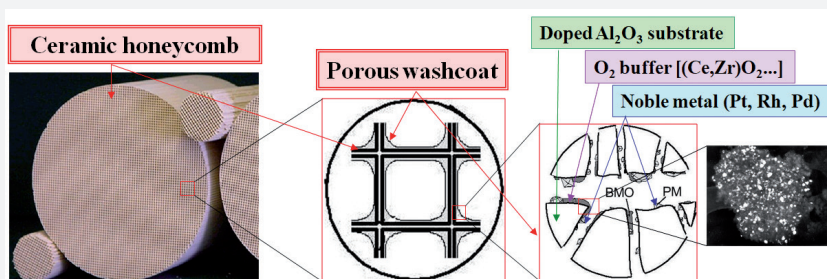
FIGURE 1 –Typical three-way catalyst for exhaust gas treatment in gasoline cars. Source: composed by J.C. Conesa using images from very different sources.
