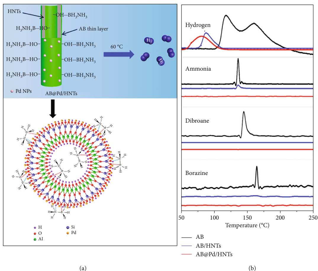
FIGURE 16: (a) The schematic representation of AB confined into the Pd/HNTs to generate H_2 at 60^\circ\text{C} . (b) MS profiles of AB, AB/HNTs, and AB@Pd/HNTs. Reproduced with permission [231]. Copyright 2020, American Chemical Society.
