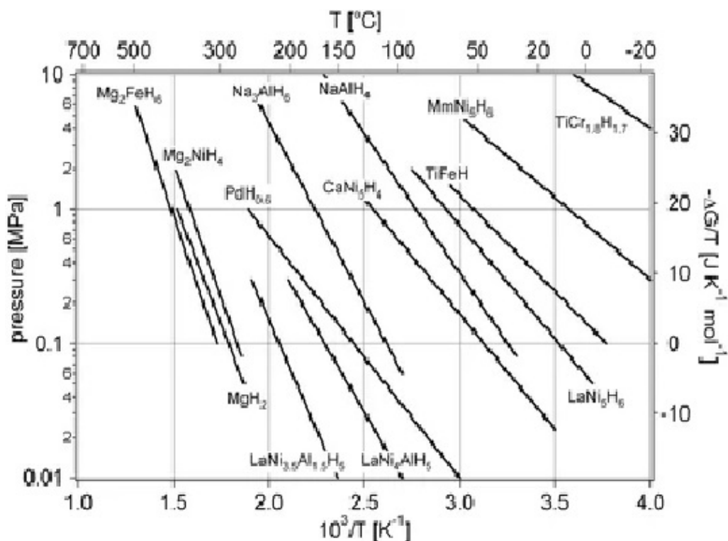
Figure 11.1: Typical Van't Hoff plots of some hydrides.
