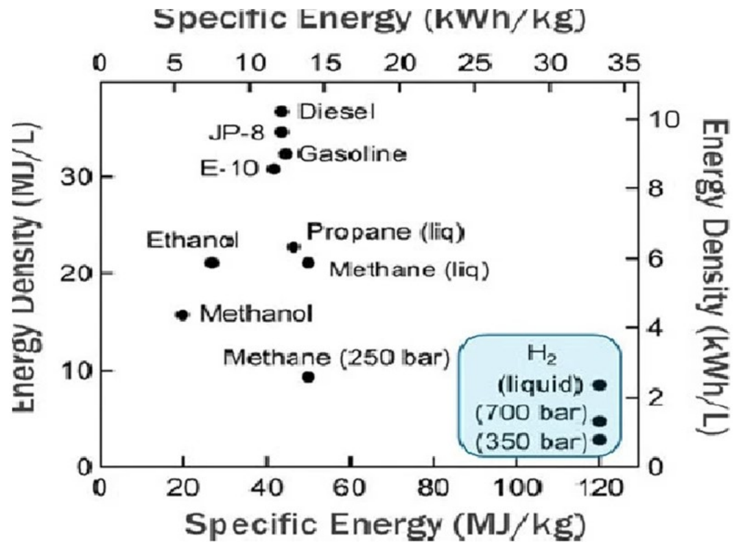
Figure.A3. Energy density and Specific Energy of Various fuels
