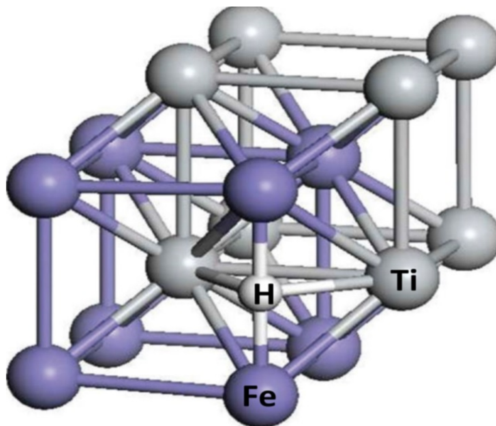
Figure 8.2: The crystal structure of FeTi
