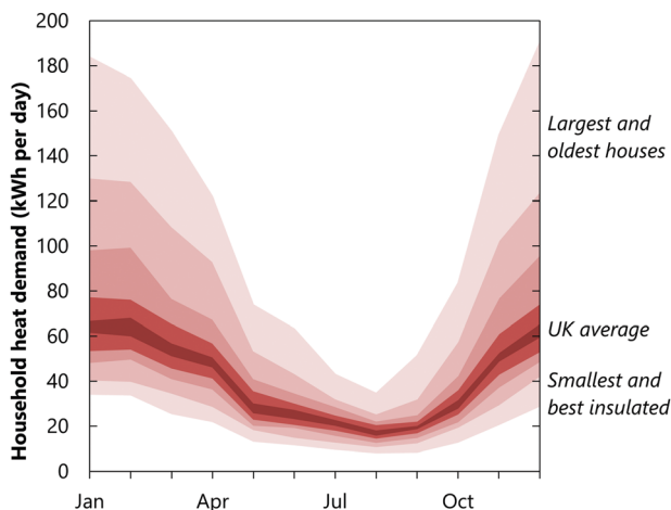
Fig. 6 Variation in British household heat demand between classes of housing for an average year. Heat demand includes space and water heating. Consumption is strongly temperature-dependent and winter peaks can be much higher in a cold year. 123
