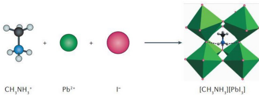
Figure 14. HOIP with an organic cation at the A-site, \text{MAPbI}_3 (orthorhombic, MA = methylammonium) [5]
