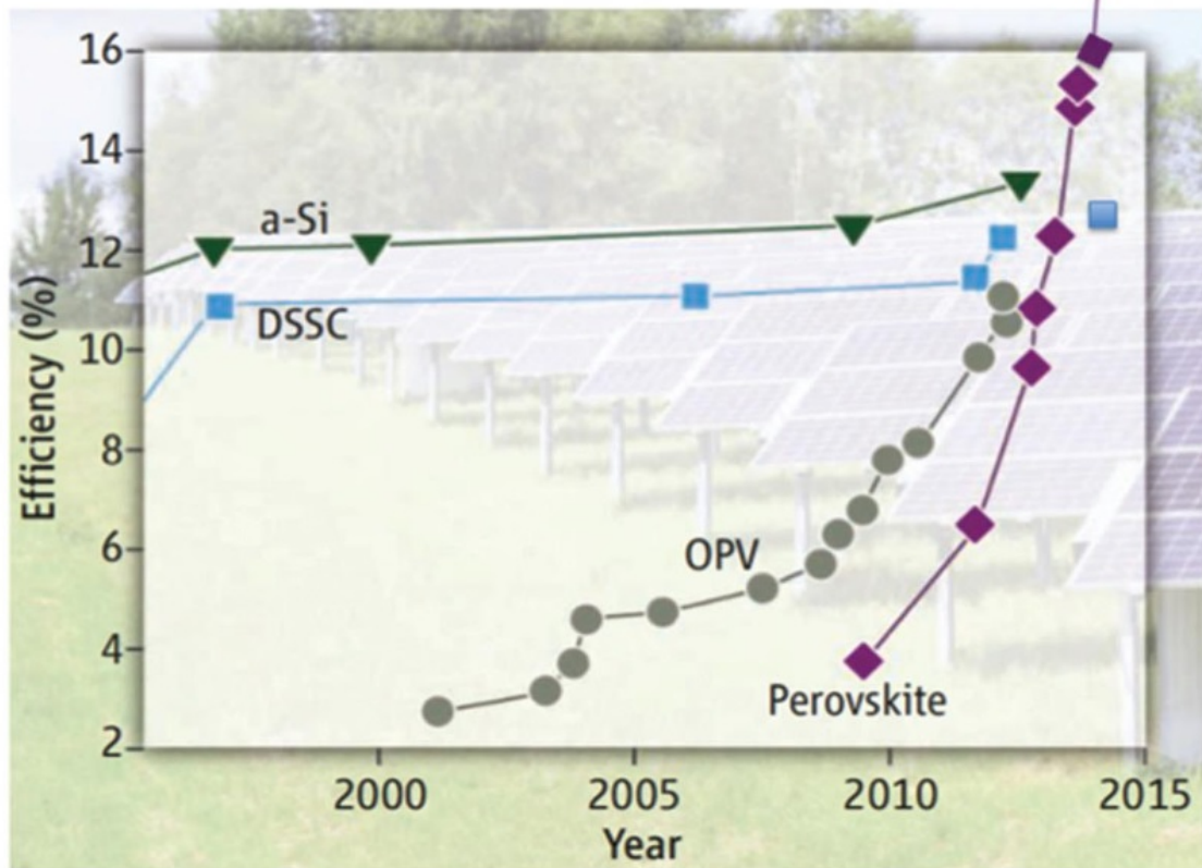
Figure 4.2: Fig.1b Typical solar cell efficiency for chosen systems with respect to the period. [reproduced from reference 7]
