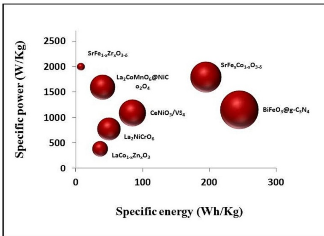
Figure 12.7: Performance metrics of Perovskite oxide supercapacitor materials. reproduced from Vyshakh Viswanath N, Johnbosco Yesuraj, Manickam Ramesh, Kibum Kim, Krishnendu Biswas, Fundamental aspects of perovskite oxides as an emerging material for supercapacitor applications and its anion intercalation mechanism - Review, Journal of Energy Storage , Volume 78, 1 February 2024, 109968
