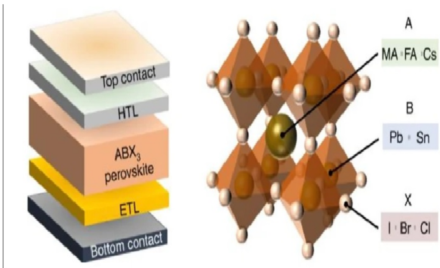
Figure 12.6: Schematic representation of perovskite solar cell, Sahil Kumar, Vishal Sharma, Neha Kumari, Gun Anit Kaur, Anirban Saha, Sapna Thakur and Mamta Shandilya, Recent advances in perovskite materials: exploring multifaceted properties for energy harvesting applications, Ionics, July 2024
