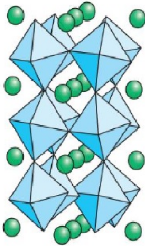
Figure 2.13: \text{GdFeO}_3 structure with 0.85 < t < 0.90 showing tilting of the \text{BO}_6 octahedra.[2]
