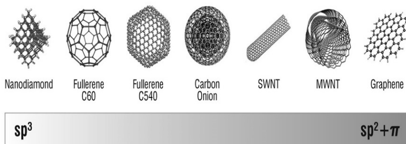
Figure 3.3: The various nanocarbons are shown based on bonding scheme
