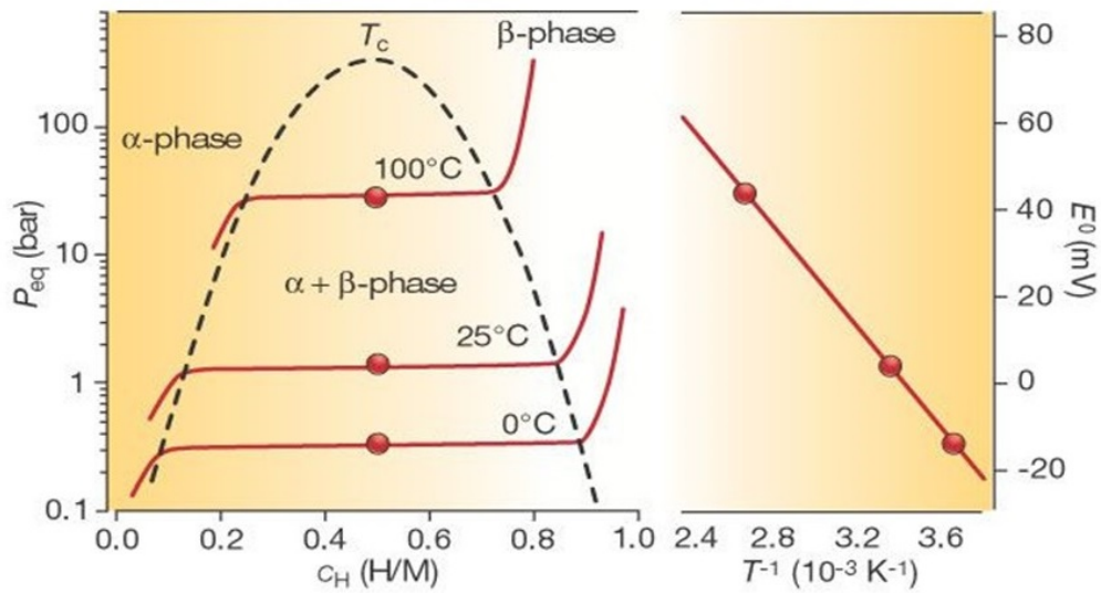
Figure 2.4: Pressure-composition-temperature curves and at the right van't Hoff plot (plot of logarithm of the equilibrium pressure versus inverse temperature for the beta phase formation; a plot to deduce the heat of hydride formation reaction). The van't Hoff plot can be used to compute the heat and entropy of the hydride formation reaction [Reproduced from ref.7]
