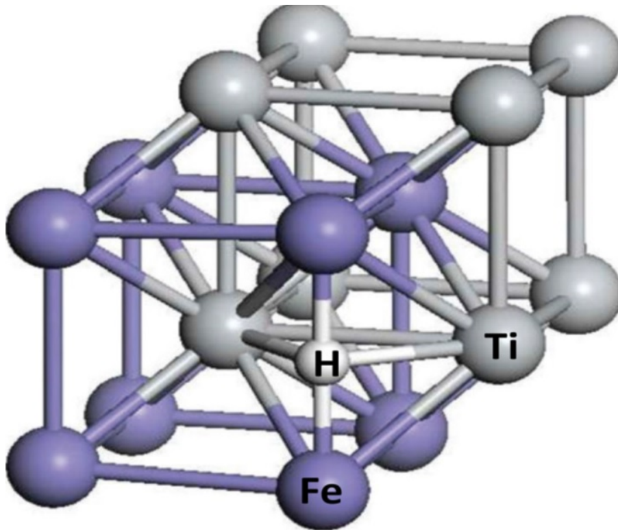
Figure 8.2: The crystal structure of FeTi
