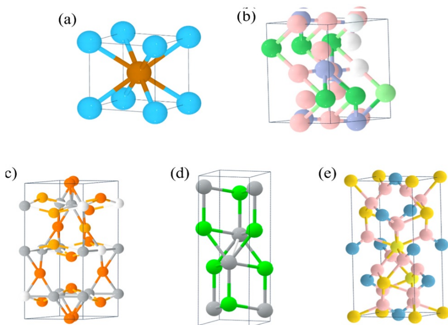
Figure 10.2: Crystal structure of (a)FeTi (b)ZrNi (c)Mg 2 Ni (d)NaAlH 4 (e)LiNH 2
