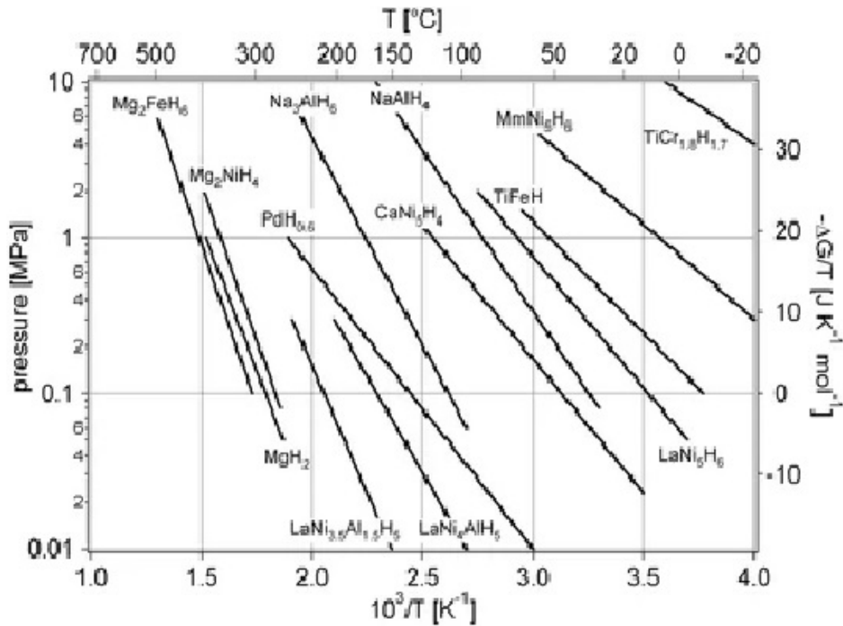
Figure 11.1: Typical Van't Hoff plots of some hydrides.
