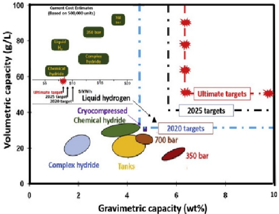
Fig A2 : Graphical representation of the Hydrogen Storage Levels of Various Solid State Materials [reproduced from Emmanuel Boateng, Aicheng Chen, Recent advances in nanomaterial-based solid-state hydrogen storage, Materials today Advances , 6, (2020), 100022]
