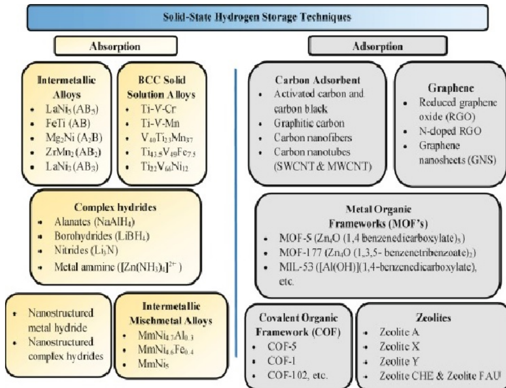
Fig A1: A birds-eye view of the solid state hydrogen storage materials. From reference Alok Kumar et al., Sustainable Energy Technologies and Assessments, 52, (2022), 102204.
