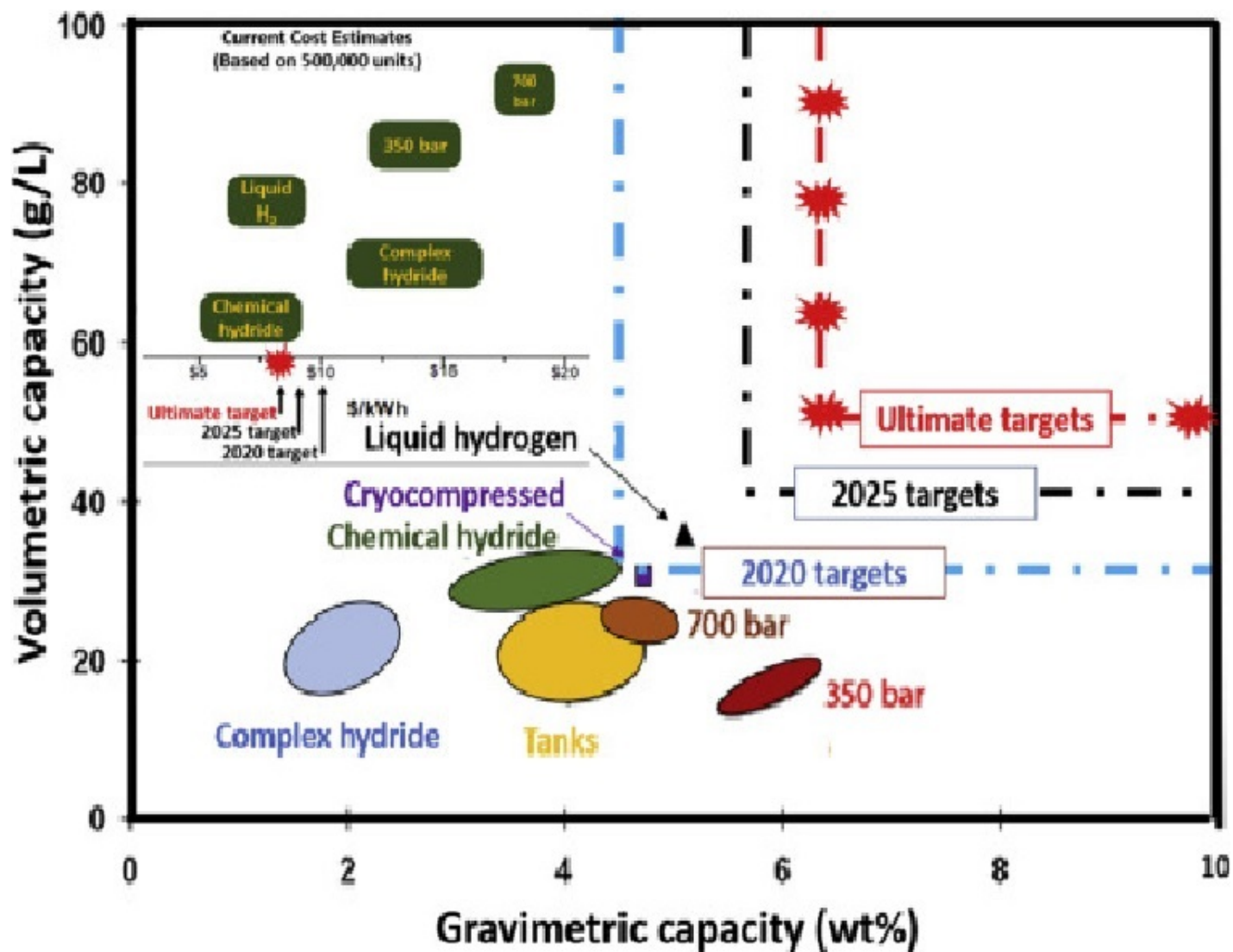
Figure 12.2: Fig A2 : Graphical representation of the Hydrogen Storage Levels of Various Solid State Materials [reproduced from Emmanuel Boateng, Aicheng Chen, Recent advances in nanomaterial-based solid-state hydrogen storage, Materials today Advances , 6 , (2020), 100022]
