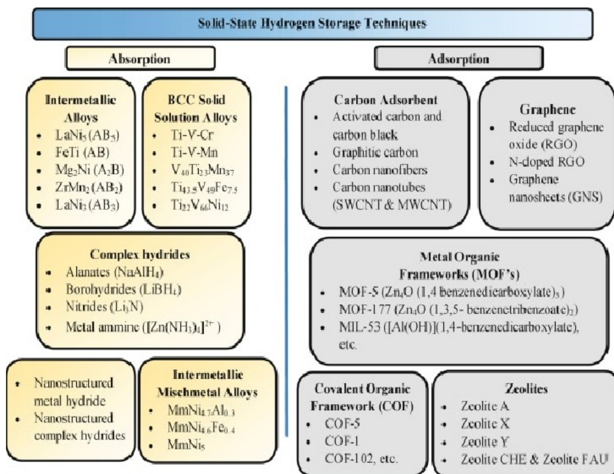
Figure 12.1: Fig A1: A birds-eye view of the solid state hydrogen storage materials. From reference Alok Kumar et al., Sustainable Energy Technologies and Assessments , 52, (2022), 102204.
