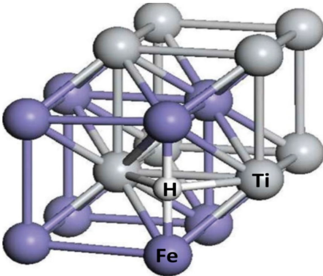
Figure 8.2: The crystal structure of FeTi
