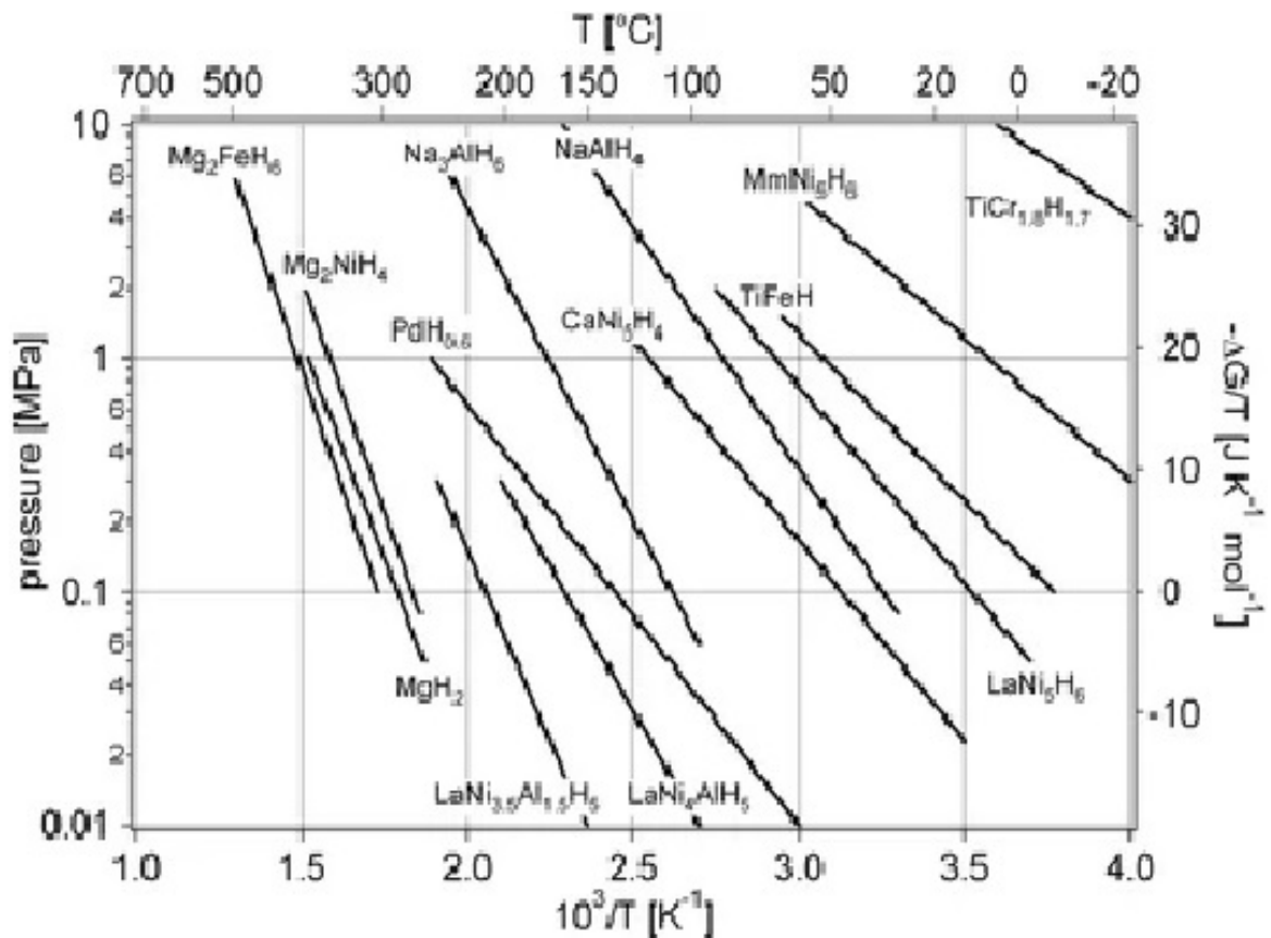
Figure 11.1: Typical Van't Hoff plots of some hydrides.
