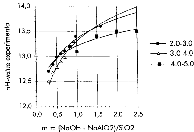
Figure 1: pH-value in the solution phase of batches with different Si/Al-ratios n in dependency of the excess alkalinity m . The data have been fitted to the function \text{pH} = a + b \log(m)
