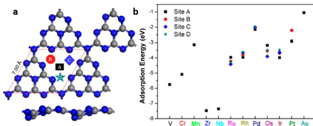
Figure 27. a) Possible adsorption sites for single metal atoms in g- C_3N_4 layer, b) Adsorption energies of various metal single atoms on available adsorption sites in the g- C_3N_4 surface. Reproduced with permission from ref. 115. Copyright 2020 American Chemical Society.
