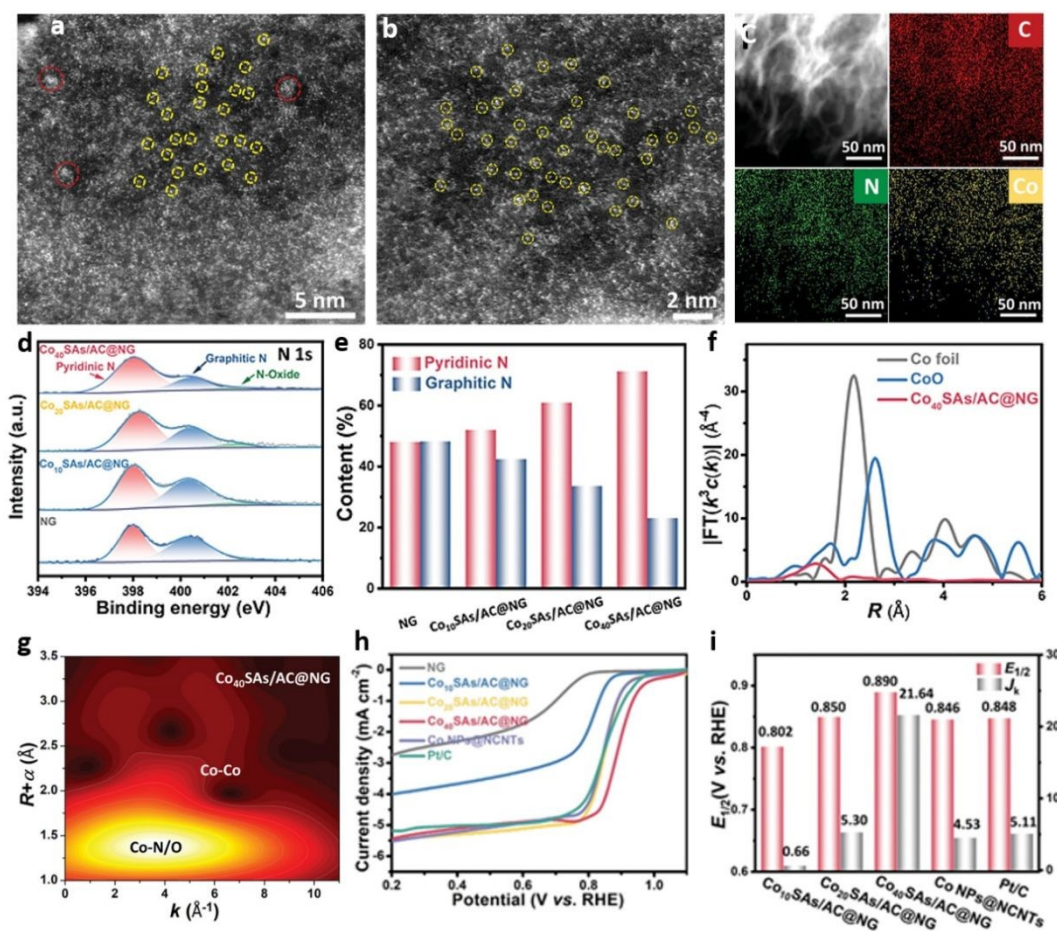
Figure 33. (a-b) HAADF-STEM images of \text{Co}_{40}\text{SAs}/\text{AC}@/\text{NG} catalyst (Aberration-corrected), (c) EDS mappings of \text{Co}_{40}\text{SAs}/\text{AC}@/\text{NG} by HAADF-STEM; Yellow and red circles represent Co single atoms and Co clusters respectively, (d) XPS N 1s spectra of NG and \text{CoSAs}/\text{AC}@/\text{NG} , (e) N content of NG and \text{CoSAs}/\text{AC}@/\text{NG} , (f-g) EXAFS spectra and WT-EXAFS plots of \text{Co}_{40}\text{SAs}/\text{AC}@/\text{NG} , (h-i) Comparison of RDE polarisation curves at a scan rate of 5 \text{ mV s}^{-1} at 1600 \text{ rpm} , J_k values at 0.85 \text{ V} & E_{1/2} values of the samples for ORR activity in \text{O}_2 -saturated 0.1 \text{ M KOH} solution. Reproduced with permission from ref. 150. Copyright 2022 John Wiley and Sons.
