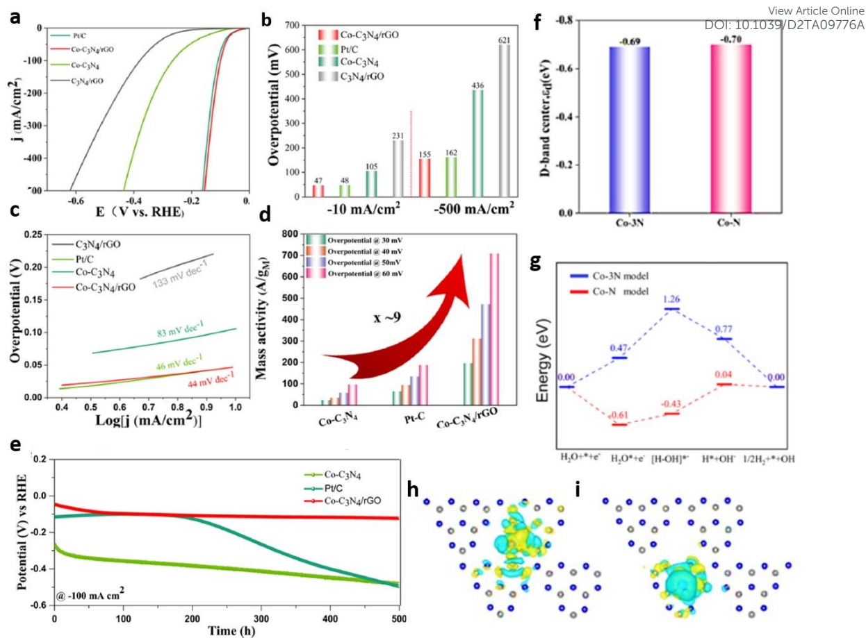
Figure 31. Data elucidation of HER activity, (a) LSV curves in 1.0 m KOH, at a scan rate of 5 \text{ mVs}^{-1} for Co- \text{C}_3\text{N}_4/\text{rGO} , Co- \text{C}_3\text{N}_4 , \text{C}_3\text{N}_4/\text{rGO} , and Pt/C, (b) Overpotential values of the developed catalysts for a current density of -10 and -500 \text{ mA cm}^{-2} , (c) Tafel plots, (d) Mass activity of the developed catalyst in comparison with Pt/C, at different overpotentials (e) Time-dependent overpotential curves of Co- \text{C}_3\text{N}_4/\text{rGO} , Co- \text{C}_3\text{N}_4 , in comparison with Pt/C. Co-N and Co-3N systems with (f) d-band centers, (g) Energy profiles, charge density differences in structures of (h) Co-N3, (i) Co-N1. Reproduced with permission from ref. 138. Copyright 2022 American Chemical Society.
