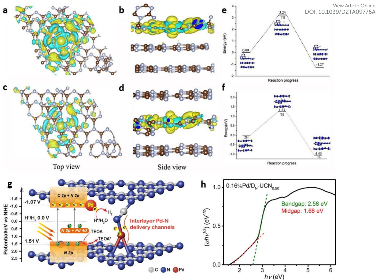
Figure 19. Charge distributions (top and side view) on Pt single atoms (a-b) on C 3 N 4 surface (SA-Pt/g-C 3 N 4 -Sur), (c-d) within the inner layer of C 3 N 4 (SA-Pt/g-C 3 N 4 -In), Energy profiles of HER over Pt atom (e) on C 3 N 4 surface and (f) within the inner layer of C 3 N 4 . Reproduced with permission from ref. 68. Copyright 2020 Elsevier. 68 , (g) Mechanism of Charge Separation, Transfer and H 2 Evolution in the photocatalyst 0.16%Pd/D N -UCN 0.50 , (h) Kubelka–Munk plot of 0.16%Pd/D N -UCN 0.50 . Reproduced with permission from ref. 70. Copyright 2022 American Chemical Society.
