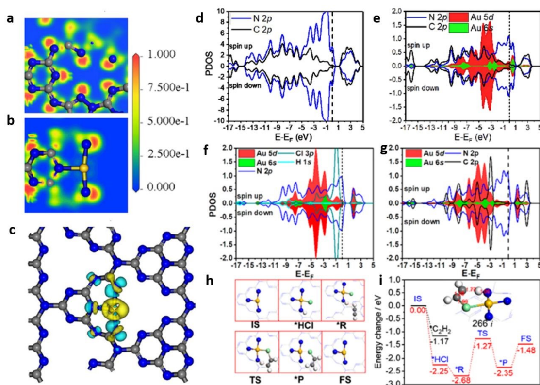
Figure 26. ELF (electron localisation function) map of (a) carbon deficient g-C 3 N 4 , (b) Au 1 /g-C 3 N 4 , (c) Charge density differences for Au atom on the g-C 3 N 4 (yellow for increasing and blue for decreasing charge density), PDOS of (d) one carbon deficient g-C 3 N 4 , (e) Au 1 /g-C 3 N 4 , Au 1 /g-C 3 N 4 (f) after HCl adsorption (g) after acetylene adsorption, (h) Reaction species configuration, (i) The reaction profile of hydrochlorination reaction
