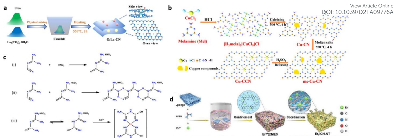
Figure 6. (a) Template free direct synthesis of La single-atoms dispersed carbon nitride (O/La-CN). Reproduced with permission from ref. 16. Copyright 2020 American Chemical Society. (b) Direct synthesis of single Cu atoms supported crystalline \text{g-C}_3\text{N}_4 (Cu-CCN) through molten salts-reflux method. Reproduced with permission from ref. 18. Copyright 2020 American Chemical Society. (c) Mechanism of supramolecular preorganization of \text{g-C}_3\text{N}_4 based cobalt SAC. Reproduced with permission from ref. 19. Copyright 2020 Elsevier. (d) Freeze drying assisted direct synthesis of erbium single atoms decorated \text{g-C}_3\text{N}_4 ( \text{Er}_1/\text{CN-NT} ). Reproduced with permission from ref. 9. Copyright 2020 John Wiley and Sons.
