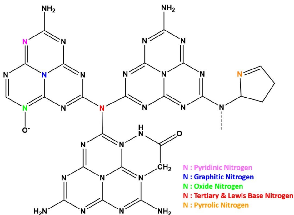
Figure 3. Types of nitrogen functionalities in g-C 3 N 4
