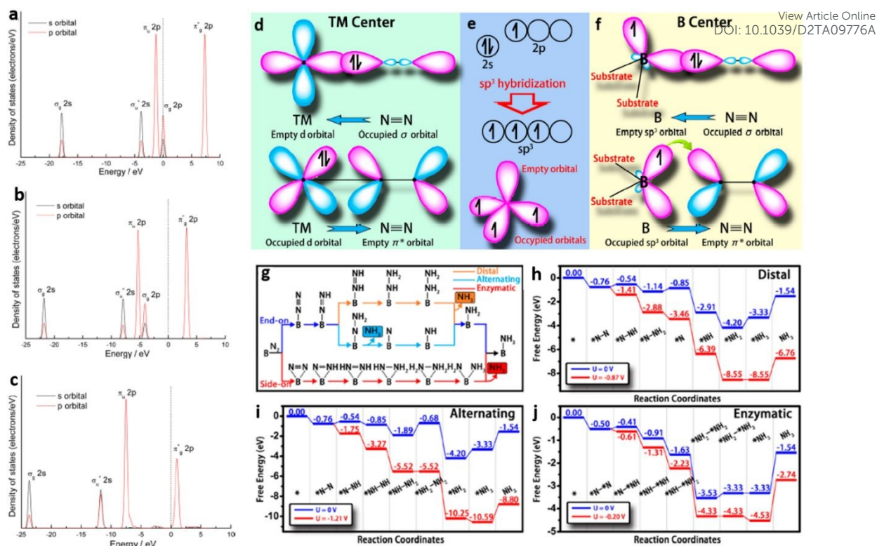
Figure 20. (a) DOS of free \text{N}_2 molecule, (b) \text{N}_2 molecule adsorbed on pure GCN and (c) \text{N}_2 molecule adsorbed on \text{M}_5\text{-Cu-CN} . Reproduced with permission from ref. 73. Copyright 2017 American Chemical Society. (d) Illustration of \text{N}_2 bonding to transition metals, (e) formation of \text{sp}^3 orbitals in B atom, (f) \text{N}_2 binding to the B atom stabilised on \text{g-C}_3\text{N}_4 , (g) distal, alternating, and enzymatic mechanisms for \text{N}_2 reduction, Free energy diagrams for (h) distal, (i) alternating, (j) enzymatic pathways for \text{N}_2 reduction on B/ \text{g-C}_3\text{N}_4 . Reproduced with permission from ref. 74. Copyright 2018 American Chemical Society.
