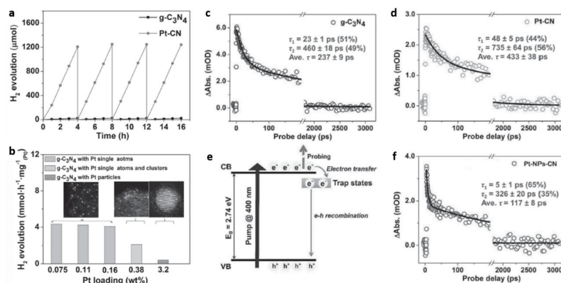
Figure 16. (a) Photocatalytic H 2 evolution with time for g-C 3 N 4 and Pt-CN, (b) Photocatalytic H 2 evolution with varying Pt content (normalised per Pt atom), Average recovery lifetime values in mOD (optical density) of (c) g-C 3 N 4 , (d) Pt-CN, (e) An illustration of the various mechanisms involved, (f) Data on TA kinetics for Pt-NPs-CN. Reproduced with permission from ref. 64. Copyright 2016 John Wiley and Sons.
