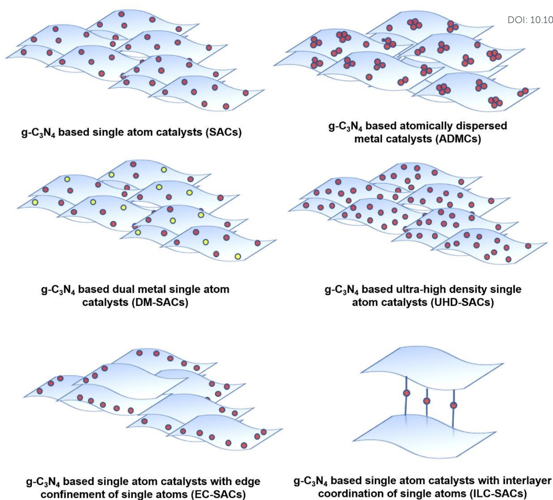
Figure 1. Various configurations of metal atom dispersions over g-C 3 N 4 matrix
