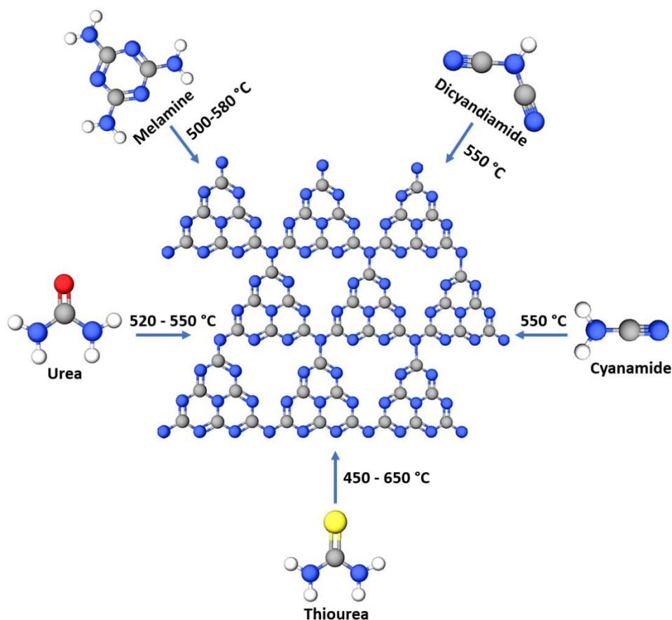
Figure 4. Synthesis of g\text{-C}_3\text{N}_4 from various nitrogen abundant precursors
