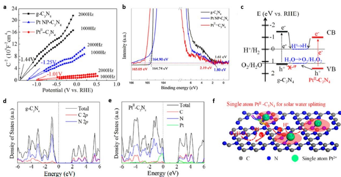
Figure 18. (a) Mott-Schottky plot of Pt^{II}-C_3N_4 in comparison with g- C_3N_4 and Pt NP- C_3N_4 , (b) UPS spectra of g- C_3N_4 , Pt^{II}-C_3N_4 & Pt NP- C_3N_4 , (c) Schematic band structure alignment, DOS of (d) g- C_3N_4 and (e) Pt^{II}-C_3N_4 , (f) Mechanistic pathways
