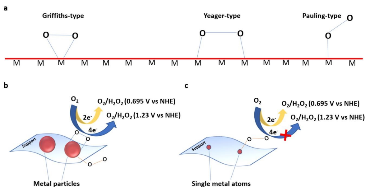
Figure 23. (a) O_2 adsorption modes on a metal surface, ORR pathways on (b) metal nanoparticles and (c) single metal atom sites.
