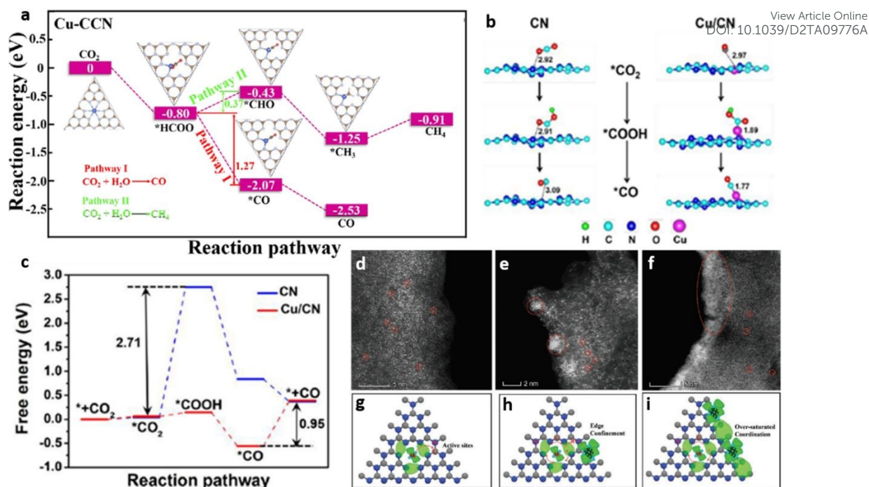
Figure 14. (a) Schematic of the photocatalytic CO 2 reduction pathway on Cu-CCN derived from DFT calculation. Reproduced with permission from ref. 18. Copyright 2020 American Chemical Society. (b) Proposed structures and CO 2 reduction pathway corresponding to CN & Cu/CN photocatalyst (c) Free energy diagram for the conversion of CO 2 to CO on CN and Cu/CN photocatalysts. Reproduced with permission from ref. 53. Copyright 2020 American Chemical Society. Aberration-corrected HAADF-STEM images of d) Ni 1 -CN, e) Ni 5 -CN, f) and Ni 10 -CN, Models showing a difference in the charge distribution of (g) Ni 1 -CN, (h) Ni 5 -CN, and (i) Ni 10 -CN. Reproduced with permission from ref. 54. Copyright 2020 John Wiley and Sons.
