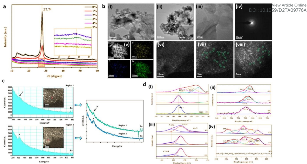
Figure 9. (a) XRD patterns of g\text{-C}_3\text{N}_4 (0%) and \text{Mo}/\text{C}_3\text{N}_4 (1–5%). Reproduced with permission from ref. 27. Copyright 2019 Elsevier. (b) Morphological analysis of O/La-CN catalyst; (i-ii) TEM images, (iii) HAADF-STEM image of the thinner region, (iv) SAED pattern, (v) HAADF-STEM EDS mapping (yellow, blue, and green color represents carbon, nitrogen and lanthanum), (vi-viii) Spherical aberration-corrected HAADF-STEM images, (c) EELS spectra of two separate labelled regions. Reproduced with permission from ref. 16. Copyright 2020 American Chemical Society. (d) XPS spectra; i) C 1s, ii) O 1s; iii) N 1s, iv) Mo 3d. Reproduced with permission from ref. 27. Copyright 2019 Elsevier.
