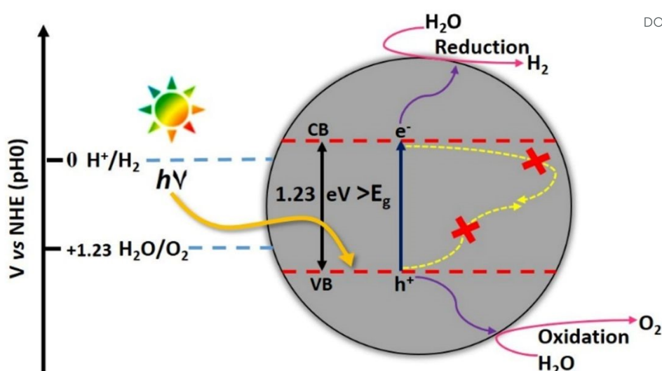
Figure 15. Schematic diagram of photocatalytic water splitting
