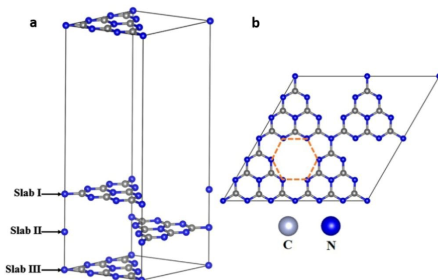
Figure 12. (a) Schematic representation of three-layer g\text{-C}_3\text{N}_4 model, (b) 2\times 2\times 1 supercell monolayer g\text{-C}_3\text{N}_4 . The highlighted ring composed of six numbers of bi-coordinated nitrogen atoms is referred to as six-fold cavity. Reproduced with permission from ref. 7. Copyright 2018 Elsevier.
