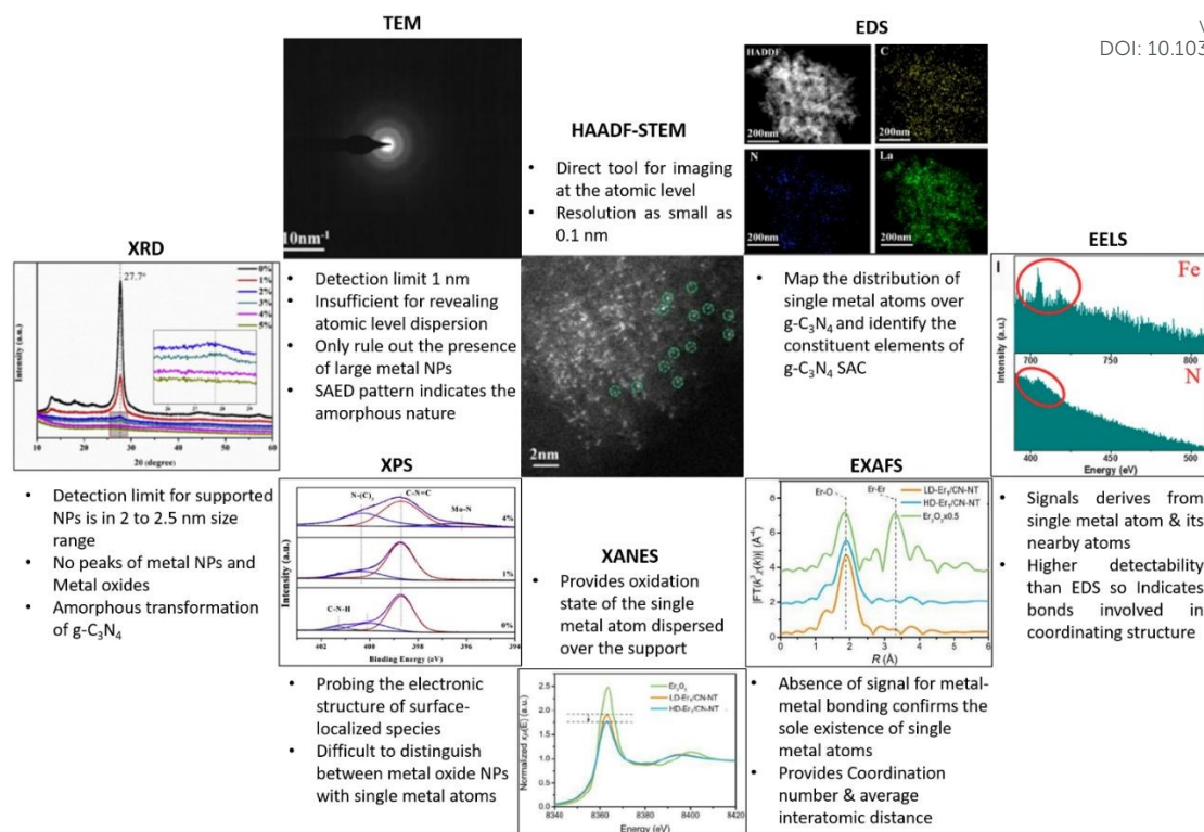
Figure 8. Various analytical tools for the characterisation g\text{-C}_3\text{N}_4 based SACs. Reproduced with permission from ref. 9. Copyright 2020 John Wiley and Sons. Reproduced with permission from ref. 16. Copyright 2020 American Chemical Society. Reproduced with permission from ref. 27. Copyright 2019 Elsevier. Reproduced from ref. 28. 28
