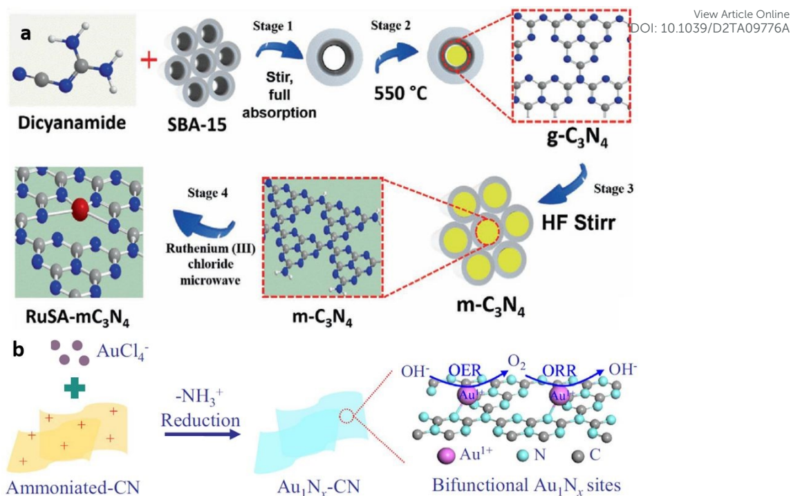
Figure 7. (a) Schematic of microwave assisted post synthetic strategy for the development of ruthenium single atoms decorated mesoporous C_3N_4 (RuSA- mC_3N_4 ) catalyst. Reproduced with permission from ref. 21. Copyright 2021 John Wiley and Sons. (b) Schematic of electrostatic adsorption mediated post synthetic strategy for Au_1N_x single-site/ C_3N_4 catalyst synthesis. Reproduced with permission from ref. 22. Copyright 2018 Elsevier.
