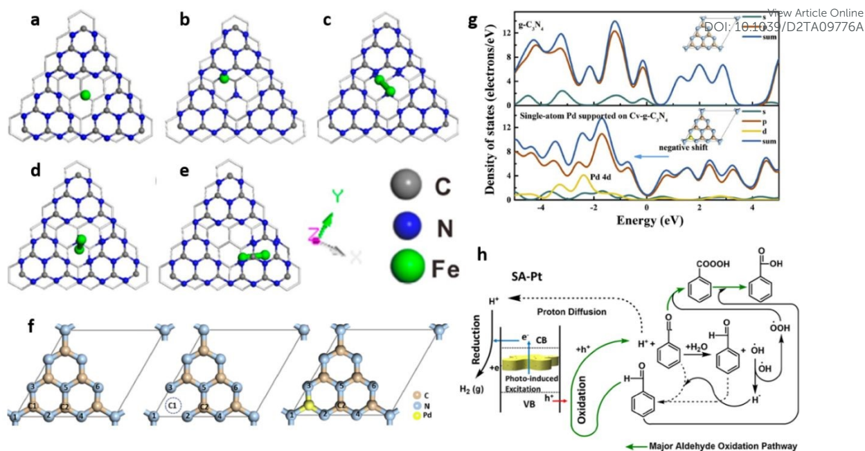
Figure 22. Structures depicting possible locations for Fe single atom and cluster over g-C 3 N 4 ; Fe Single atom in (a) 6-fold cavity centre, (b) interlayer. Fe cluster sites in the interlayer (c), Site 1, (d) Site 2 (e) Site 3. Reproduced with permission from ref. 84. Copyright 2018 American Chemical Society. (f) The carbon vacancies and single atom site of Pd in g-C 3 N 4 and (g) corresponding DOS. Reproduced with permission from ref. 90. Copyright 2021 Elsevier. (h) Schematic diagram representing the mechanism of benzaldehyde oxidation and associated H 2 evolution with photoinduced electron and hole transfer. Reproduced with permission from ref. 91. Copyright 2021 Elsevier.
