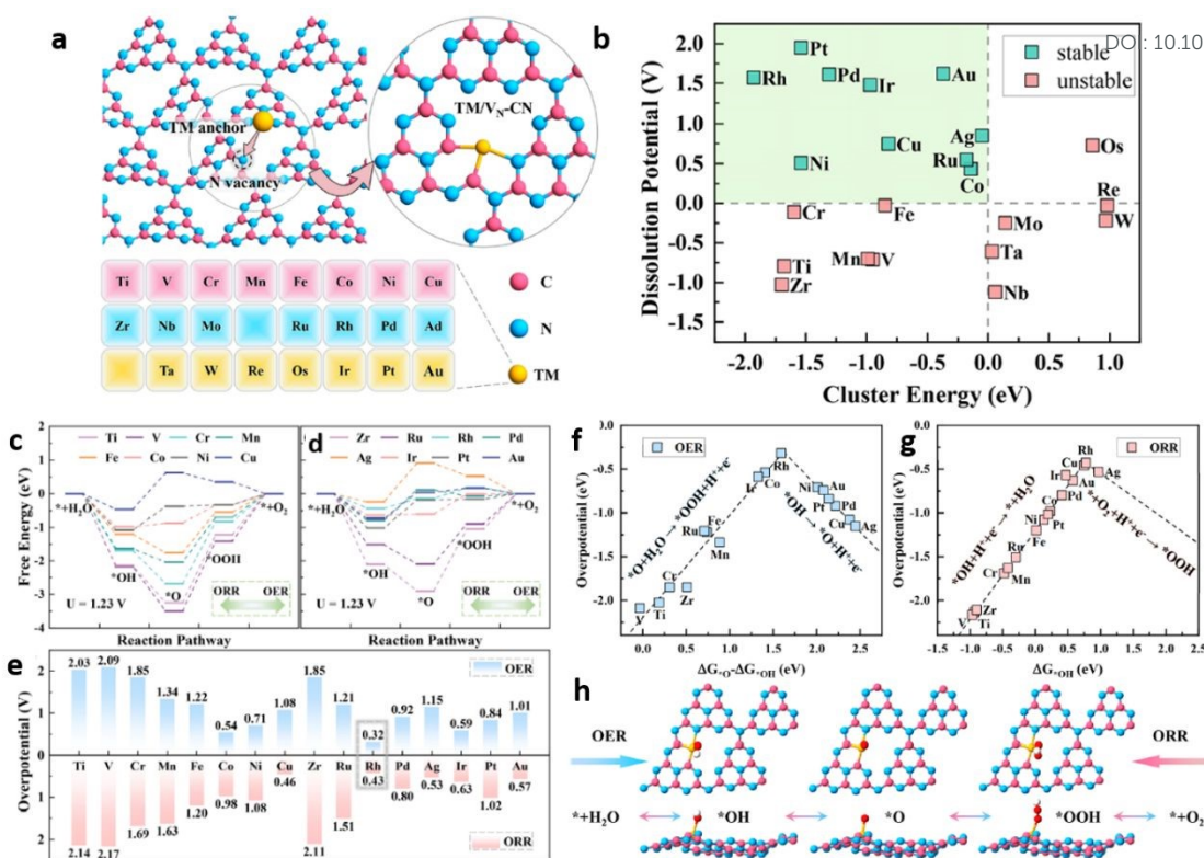
Figure 32. (a) Schematic representation of various transition metals (TM) based SACs on VN-CN, (b) Stability of TM/V N -CN based on Cluster energy ( E_{\text{Clus}} < 0 eV) and dissolution potential ( U_{\text{diss}} > 0 eV), The free energy diagrams of TM/VN-CN (c) from Ti to Cu and (d) from Zr to Au related to both OER and ORR at the equilibrium potential of 1.23, (e) The OER and ORR overpotentials of TM/VN-CN (from Ti to Au), The volcano plots of (f) OER ( -\eta_{\text{OER}} vs \Delta G^*O - \Delta G^*OH ) and (g) ORR ( -\eta_{\text{ORR}} vs \Delta G^*OH ) on TM/VN-CN, (h) OER and ORR intermediate structures adsorbed on Rh/VN-CN. Reproduced with permission from ref. 10. Copyright 2021 American Chemical Society.
