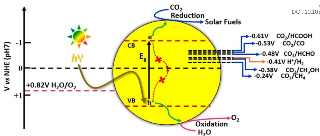
Figure 13. Schematic illustration of photocatalytic carbon dioxide reduction
