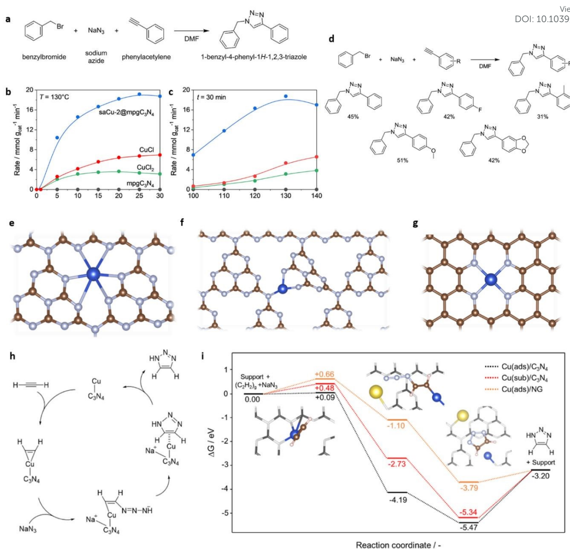
Figure 28. (a) Reaction scheme of cycloaddition, (b-c) The comparison of catalytic performance of mpgC 3 N 4 , CuCl 2 , CuCl, and saCu-2@mpgC 3 N 4 with respect to (b) time and (c) temperature, (e-g) The structural model for the Cu coordination in Cu-based SACs (e) Cu adsorbed in the heptazinic pore of C 3 N 4 (Cu(ads)/C 3 N 4 ), (f) Cu substituted the carbon in C 3 N 4 (Cu(sub)/C 3 N 4 ), and (g) Cu adsorbed on N-doped graphene at its dicarbon vacancy (Cu(ads)/NG), (h) Proposed reaction mechanism for click cycloaddition over supported Cu 1 active sites, (i) Reaction free-energy profile for (Cu(ads)/C 3 N 4 ), (Cu(sub)/C 3 N 4 ), and (Cu(ads)/NG) at 130 °C (inset: Structures of intermediates formed over Cu(ads)/C 3 N 4 ). Reproduced with permission from ref. 117. Copyright 2022 The Authors. Published by American Chemical Society.
