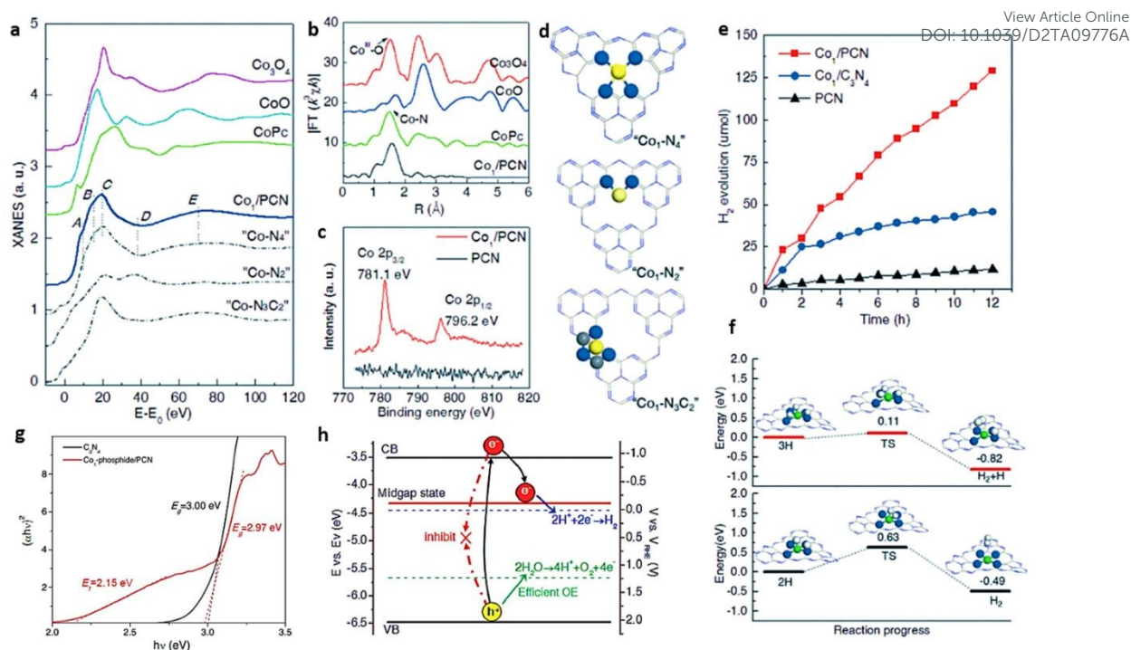
Figure 17. (a) XANES (Co K-edge) spectra of Co 1 /PCN in comparison with standards and possible atomic configurations (b) Fourier spectra of Co 1 /PCN in comparison with standards (c) XPS Co 2p spectra of Co 1 /PCN and C 3 N 4 , (d) Model structures of “Co 1 -N 4 ”, “Co 1 -N 2 ”, “Co 1 -N 3 C 2 ” with blue, yellow and grey spheres representing N, Co and C atoms, respectively, (e) H 2 evolution with time under simulated solar irradiation, (f) Energy diagram of Co 1 -N 4 for H 2 evolution on single-sites with the transition state of the reaction TS-(H+H→H 2 ). N (blue), Co (green) and H (white) spheres. Reproduced with permission from ref. 24. Copyright 2017 John Wiley and Sons. (g) The Tauc plot of the g-C 3 N 4 and Co 1 phosphide/PCN catalysts (h) Electronic band structure of Co 1 -phosphide/PCN catalyst. Reproduced with permission from ref. 65. Copyright 2017 John Wiley and Sons.
