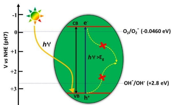
Figure 21. Schematic of the photocatalytic process
