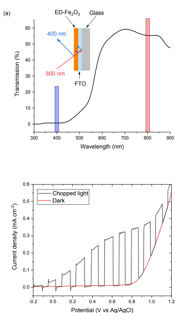
Figure 2: (a) UV-Vis in transmission of the \alpha - \text{Fe}_2\text{O}_3 electrode used for SHG experiments. Inset, experimental geometry for reflection SHG experiments, highlighting the absorption of SHG photons (blue) from the buried interface by the layer of hematite on commercial FTO-coated glass. (b) Chopped light ( 15 \text{ mW cm}^{-2} , 365 nm) and dark linear sweep voltammograms (LSVs) at 10 \text{ mV s}^{-1} of \alpha - \text{Fe}_2\text{O}_3 electrode in 0.1 M NaOH.
