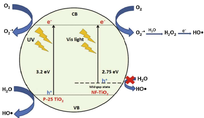
Fig. 27. Role of various reactive oxidation species during the photocatalysis process of N-F doped \text{TiO}_2 .
