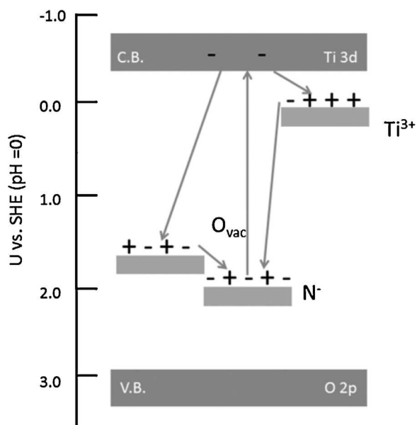
Fig. 26. Mechanism of electron transfer from either \text{Ti}^{3+} or oxygen vacancies in N-F doped \text{TiO}_2 explained using photo-electrochemical studies.
