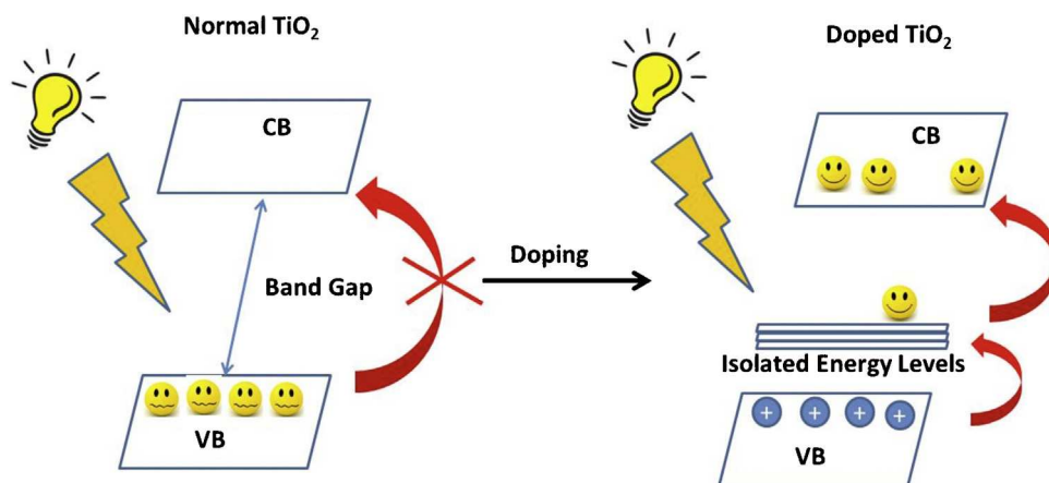
Fig. 22. Schematic mechanism of band gap narrowing in anion doped \text{TiO}_2 .
