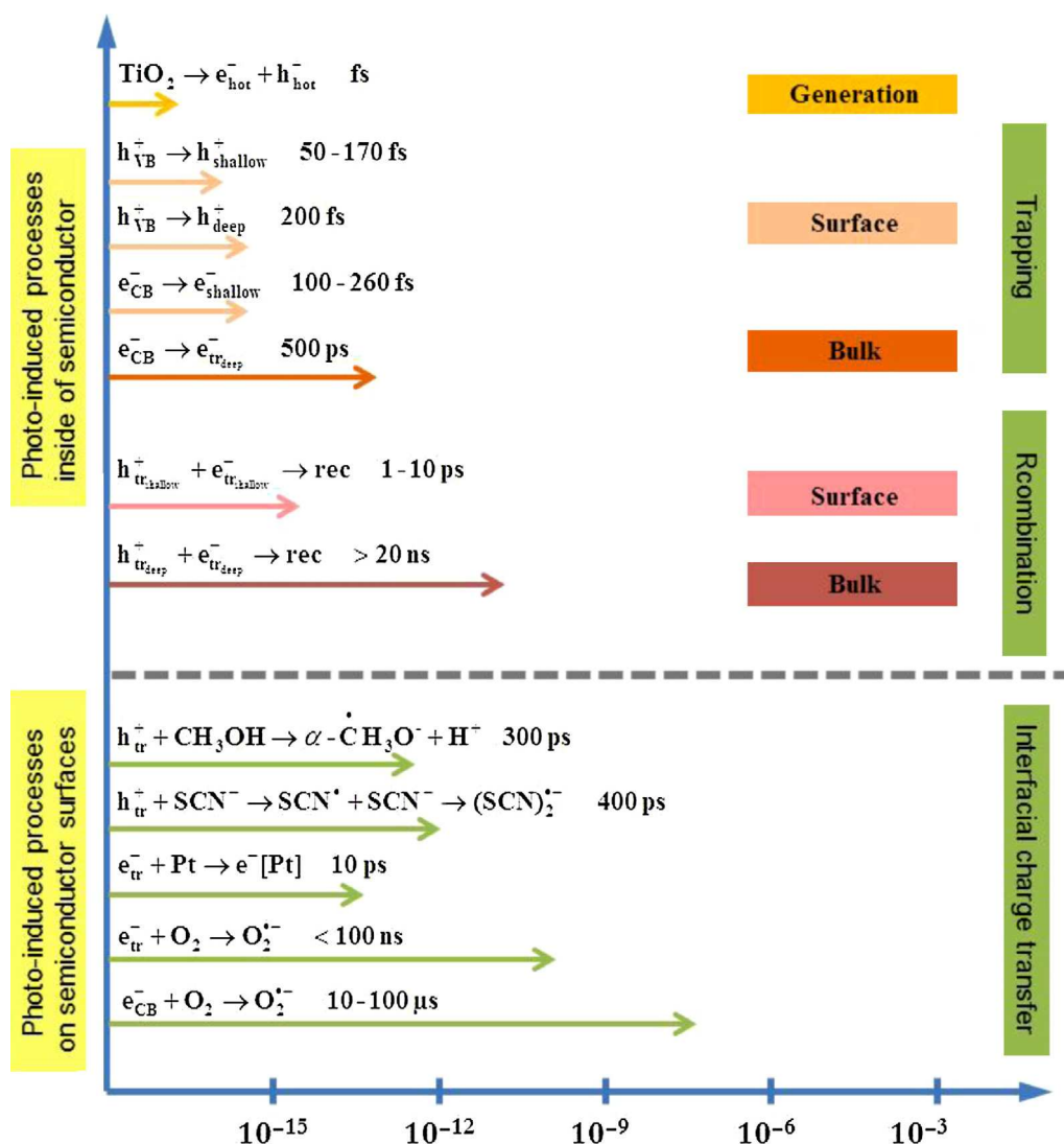
Scheme 1. Various steps involved in \text{TiO}_2 photocatalysis.
