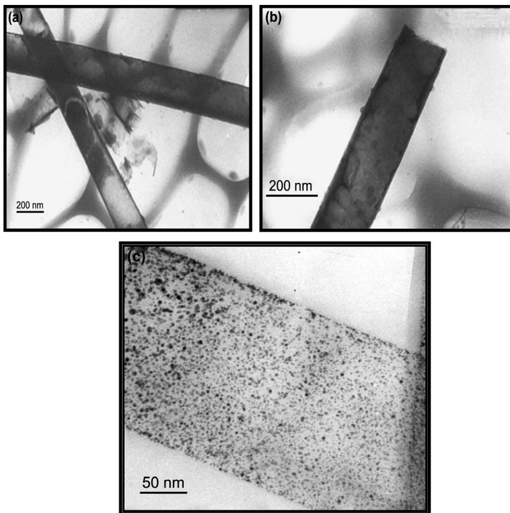
Fig. 3. TEM images of the nitrogen containing carbon nanotubes: (a) at lower magnification; (b) at higher magnification image of the individual nanotube (an arrow indicating the open end of the tube) and (c) Pt filled nitrogen containing carbon nanotubes.
