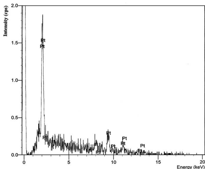
Fig. 4. EDX pattern of Pt/N-CNT electrode.
