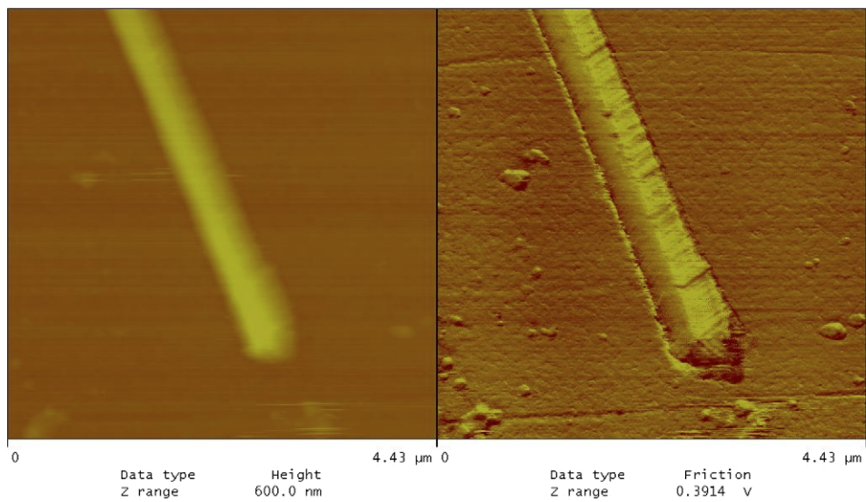
Fig. 2. AFM image of the nitrogen containing carbon nanotubes.
