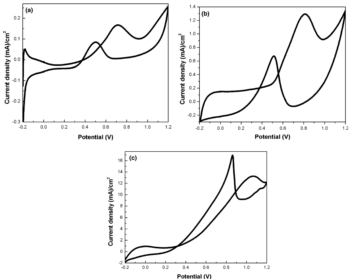
Fig. 5. Cyclic voltammograms of (a) pure Pt; (b) Pt/Vulcan (E-TEK) and (c) Pt/N-CNT in 1 M \text{H}_2\text{SO}_4 /1 M \text{CH}_3\text{OH} run at 50 \text{ mV s}^{-1} .
