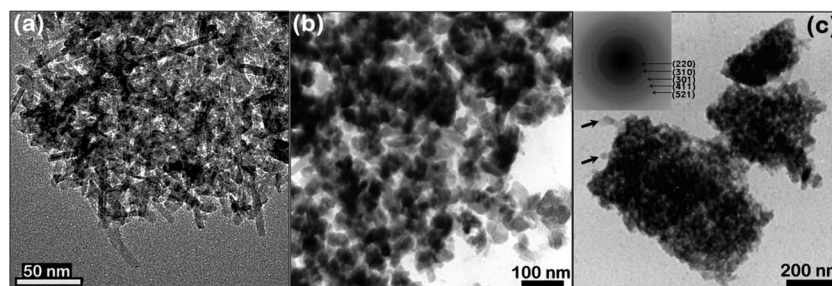
Fig. 7 HRTEM image of Crypt-A400 (a) and TEM images of Crypt-B400 (b) and Crypt-C400 (c). Inset in image (c) shows SAED pattern acquired on Crypt-C400, and arrow marks indicate the projecting nanorods.
