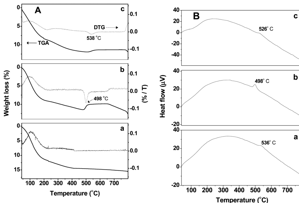
Fig. 3 TGA (A) and DTA (B) profiles of birnessite samples recorded in air atmosphere. (a) Birn-A; (b) Birn-B; (c) Birn-C.
