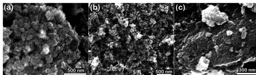
Fig. 4 SEM images of birnessite samples. (a) Birn-A; (b) Birn-B; (c) Birn-C.
