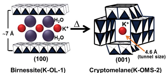
Fig. 1 Schematic of birnessite and cryptomelane structures.
