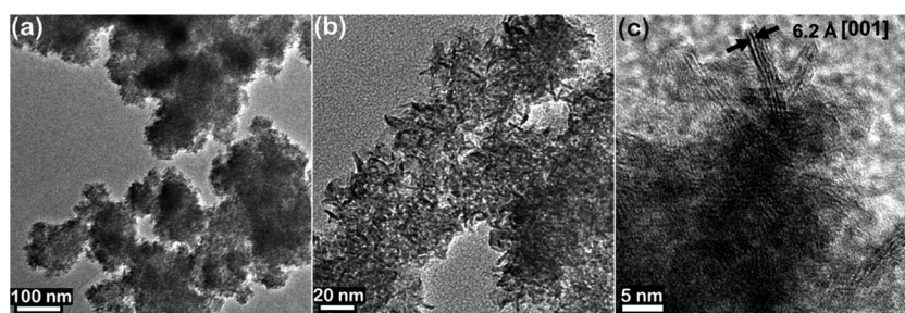
Fig. 6 HRTEM images of Birn-A. (a) and (b) low magnification and (c) lattice-resolved TEM images of Birn-A.
