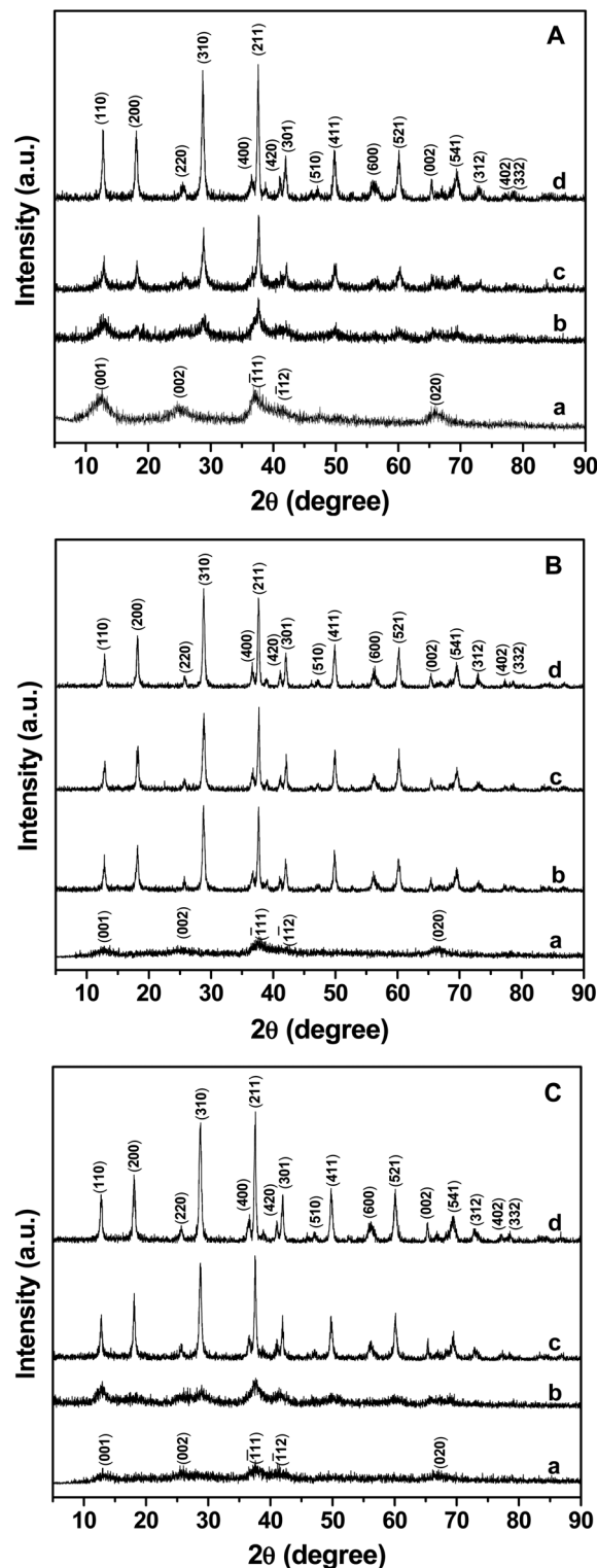
Fig. 2 Powder XRD patterns of birnessites and cryptomelanes and A, B or C denotes the method of preparation. (a) Birnessite; (b) Crypt-400(2h); (c) Crypt-400; (d) Crypt-600.
