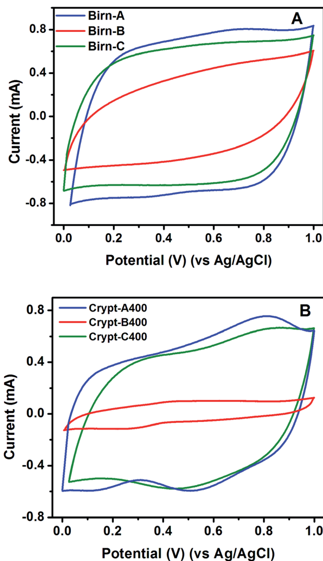
Fig. 13 Cyclic voltammograms of birnessite (A) and cryptomelane (B) carbon composite electrodes, run in 0.1 M aqueous Na 2 SO 4 solution at a scan rate of 10 mA s -1 .
