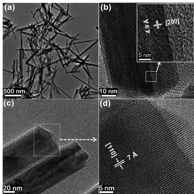
Fig. 8 HRTEM images of Crypt-A600. (a) low magnification image; (b) TEM image of a nanorod and its lattice-resolved image of a side portion (inset); (c) TEM image of edges of nanorods; (d) lattice-resolved TEM image of an edge of the nanorod in (c).
