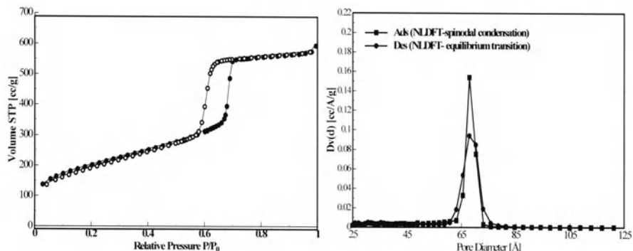
Figure 8.4 Nitrogen adsorption/desorption at 77.35 K in ordered SBA-15 and NLDFT pore size distributions (NLDFT for N_2 /silica [46]) from adsorption- (spinodal condensation) and desorption (equilibrium transition) branch. From [49].
