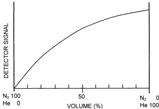
Figure 15.6 Thermal conductivity bridge response.
