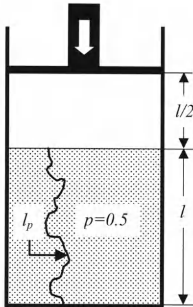
Figure 6.2 Piston displacement forcing gas to flow along a tortuous path through a packed powder bed.
