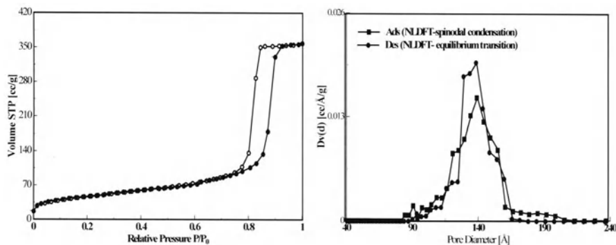
Figure 8.5 Nitrogen adsorption/desorption at 77.35 K in controlled pore glass and NLDFT pore size distribution (NLDFT for N_2 /silica [46]) from adsorption- (spinodal condensation) and desorption (equilibrium transition) branch. From [49].
