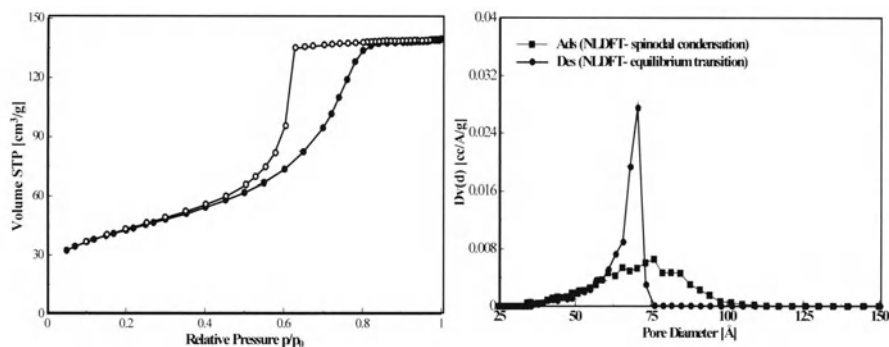
Figure 8.6 Nitrogen adsorption/desorption at 77.35 K in porous Vycor® glass and NLDFT pore size distribution (NLDFT for N_2 /silica [46]) from adsorption- (spinodal condensation) and desorption (equilibrium transition) branch. From [49].
