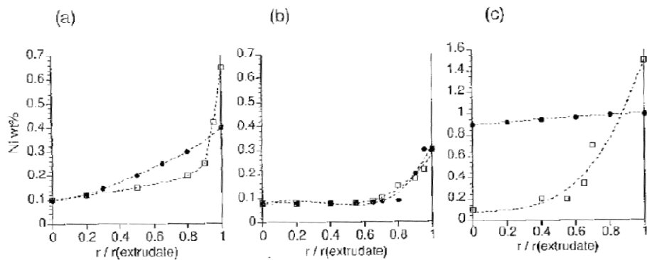
Figure 4.2 Profiles of nickel content in spherical extrudates before drying (black circles) and after drying (white squares). The origin of axis x corresponds to the center of the extrudate. (a) Low drying rate to 110°C; (b) high drying rate to 110°C; and (c) drying at 200°C. (Data have been collected from [41] (a and b) and [31] (c).)
