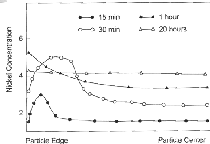
Impregnation of alumina with aqueous Ni(NO 3 ) 2
