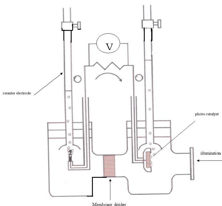
Figure 1.2: Typical reactor design conventionally employed for the photo-splitting of water.
