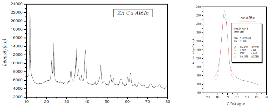
Fig 4.1.2 (e): XRD pattern for Zn Cu Al&In.
