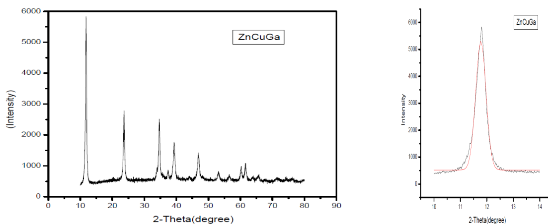
Fig 4.1.2 (b): XRD pattern for Zn Cu Ga
