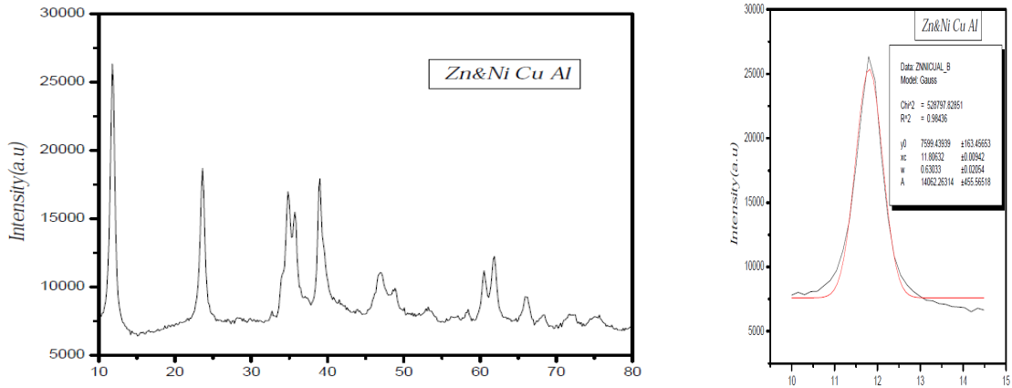
Fig 4.1.2 (d): XRD pattern for Zn&Ni Cu Al.
