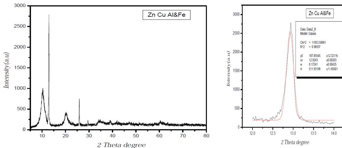
Fig 4.1.2 (f): XRD pattern for Zn Cu Al&Fe.
