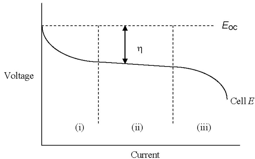
Figure 2. Typical polarization curve for a fuel cell: voltage drops due to: (i) surface reaction kinetics; (ii) electrolyte resistance; and (iii) reactant/product diffusion rates [reproduced from ref. 9].
