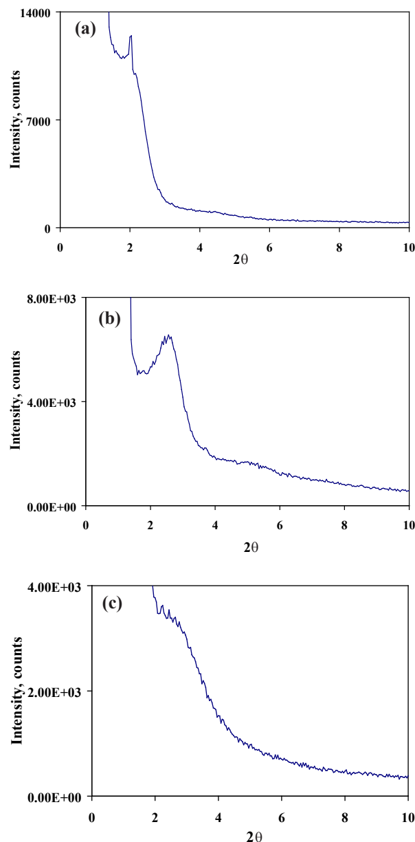
Fig. 1. (a) XRD pattern of mesoporous TiO 2 as synthesized (b) calcined at 823 K (c) calcined at 923 K.
