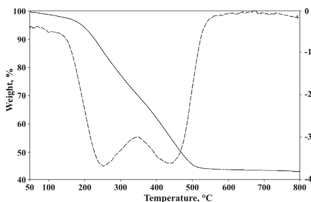
Fig. 4. Thermogravimetric analysis of mesoporous titania.
