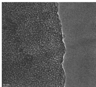
Fig. 3. TEM image of mesoporous titania calcined at 823 K.
