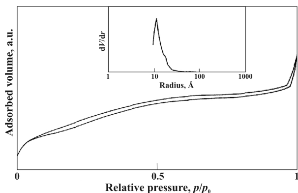
Fig. 2. Nitrogen adsorption-desorption isotherms of mesoporous titania.
