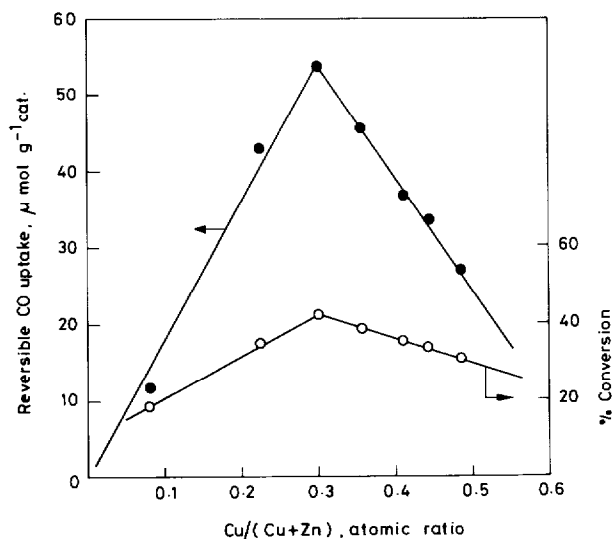
Fig. 1. Reversible carbon monoxide uptake at 25°C and cyclohexanol conversion at 250°C as a function of Cu/(Cu+Zn) atomic ratio.
